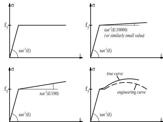
Figure 3. Material model
