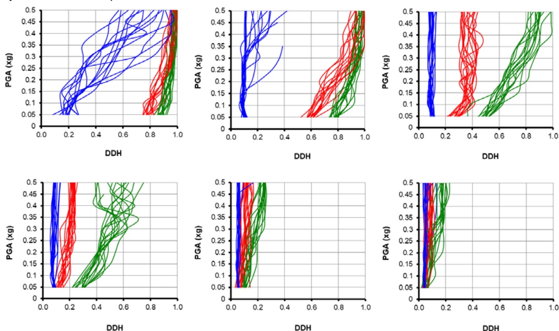
Figure 4. DDH index in function of PGA for analyzed frames (R1 to R6 consequently)
