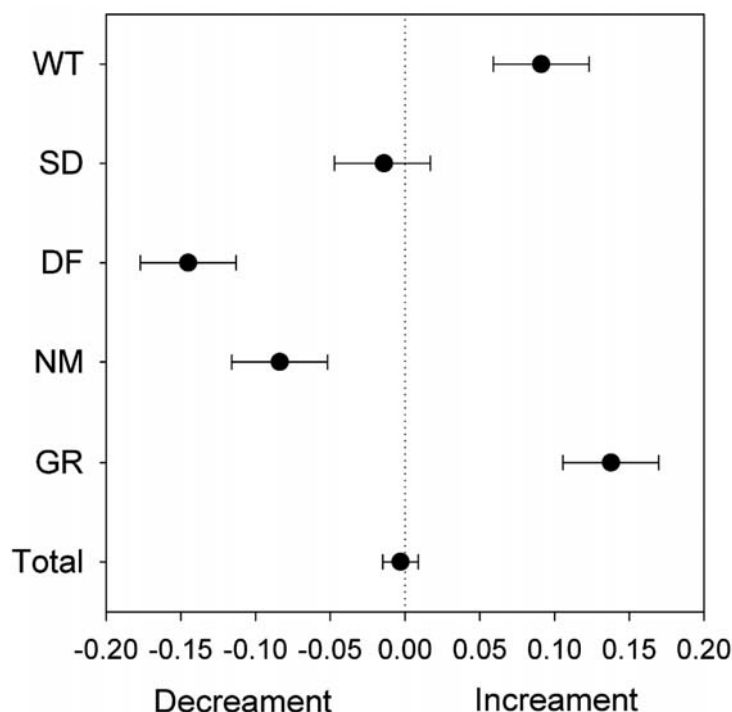
Figure 1b. Meta-analysis of the predictor variables. The dots in the figure show the mean effect sizes and the horizontal bars the range of 95% confidence interval. Thus, if the bar crosses the vertical dotted line (effect size=0) the mean is not significantly different from zero
