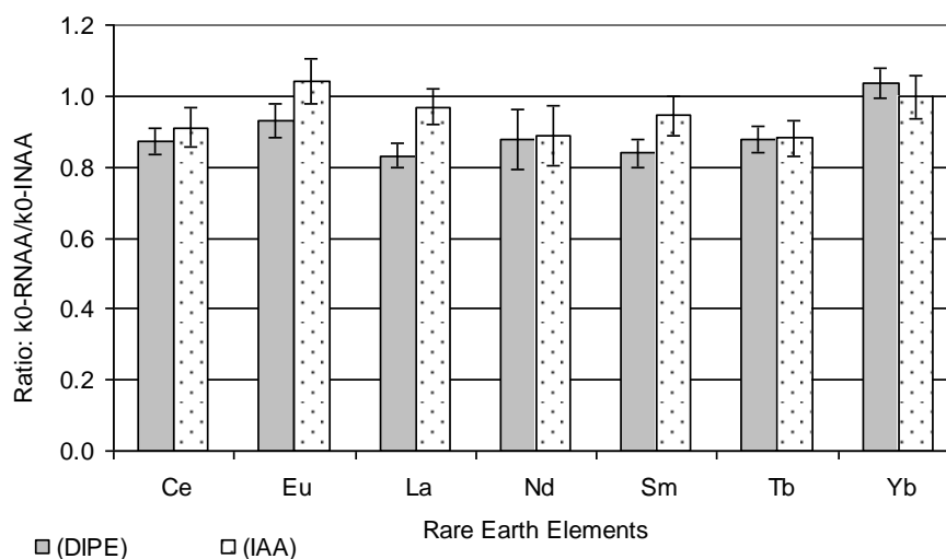
Fig. 1. Ratio between k_0 -RNAA (extraction into DIPE and IAA) and k_0 -INAA for REE in hematite [36]
