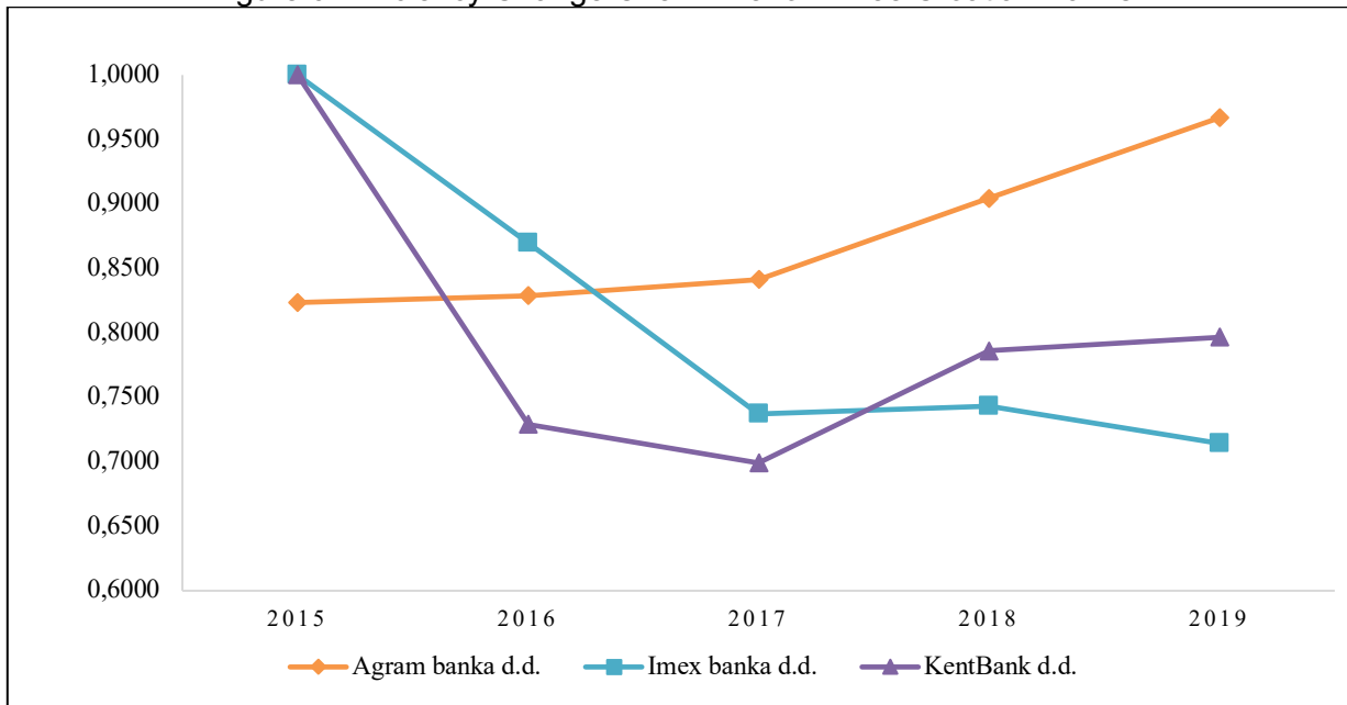
Figure 6. Efficiency Change Over Time for Three Croatian Banks
