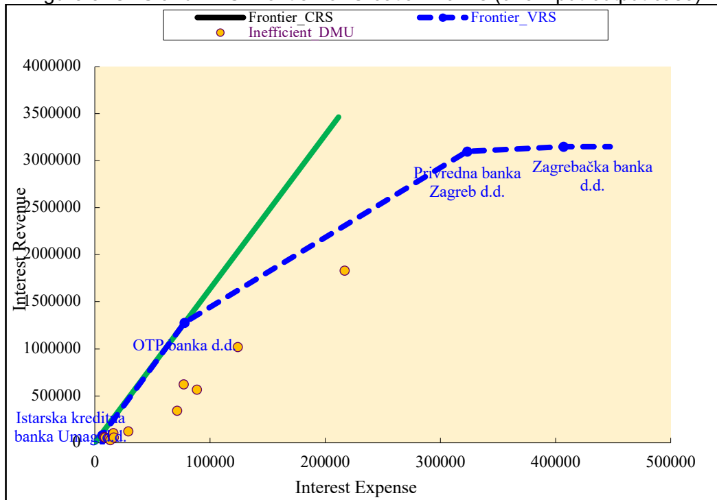
Figure 5. CRS and VRS Frontier for Croatian Banks (one input-output case)
