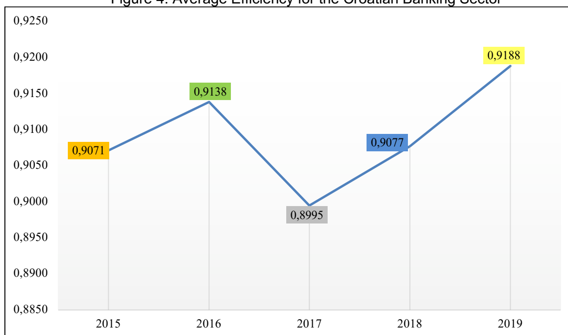
Figure 4. Average Efficiency for the Croatian Banking Sector
