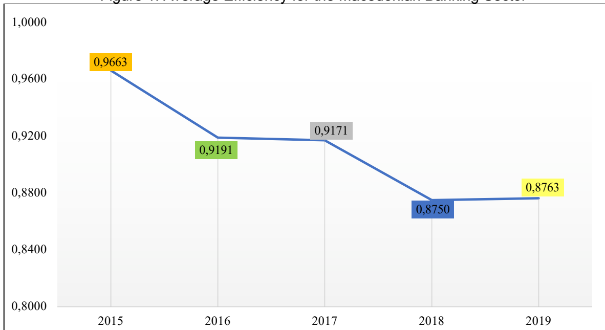
Figure 1. Average Efficiency for the Macedonian Banking Sector
