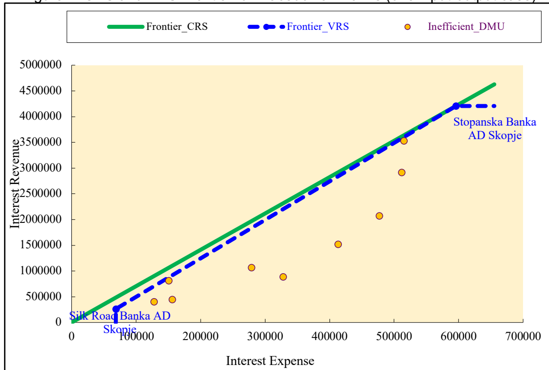
Figure 2. CRS and VRS Frontier for Macedonian Banks (one input-output case)
