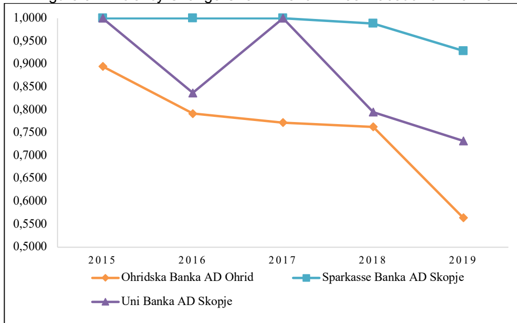
Figure 3. Efficiency Change Over Time for Three Macedonian Banks
