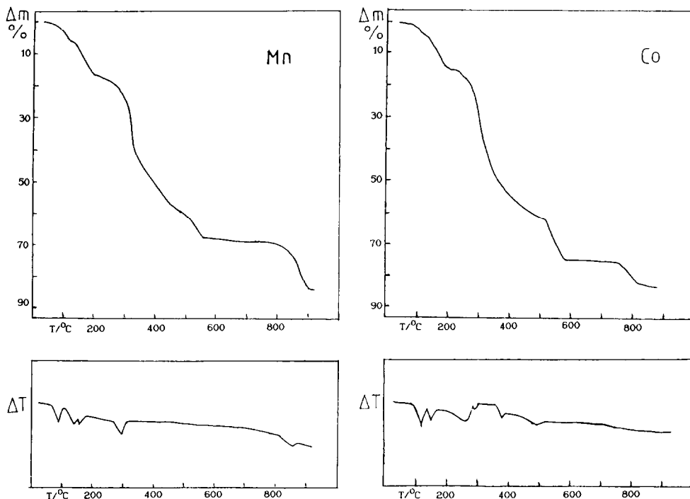
Fig. 1. TG and DTA curves of (\text{RH})_2\text{M}(\text{SO}_4)_2 \cdot 4\text{H}_2\text{O} (where M is Mn or Co).
