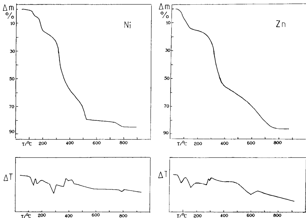
Fig. 2. TG and DTA curves of (\text{RH})_2\text{M}(\text{SO}_4)_2 \cdot 4\text{H}_2\text{O} (where M is Ni or Zn).
