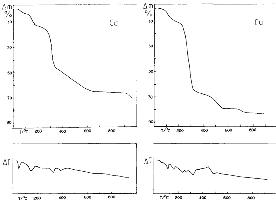
Fig. 3. TG and DTA curves of (\text{RH})_2\text{M}(\text{SO}_4)_2 \cdot 4\text{H}_2\text{O} (where M is Cd or Cu).
