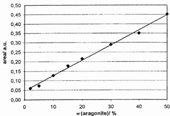
Fig. 3. The relationship between the integral intensity of the analytical band ( 1090-1075\text{ cm}^{-1} ) and the mass fraction ( w ) of aragonite in the aragonite-calcite mixtures
