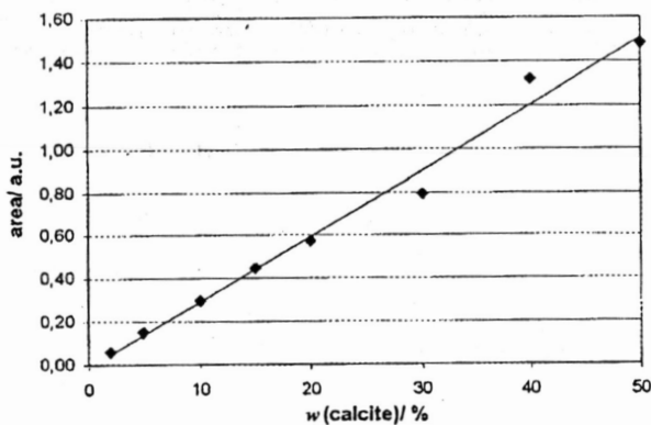
Fig. 5. The relationship between the integral intensity of the analytical band ( 740\text{--}724.5\text{ cm}^{-1} ) and the mass fraction ( w ) of calcite in the calcite–aragonite mixtures
