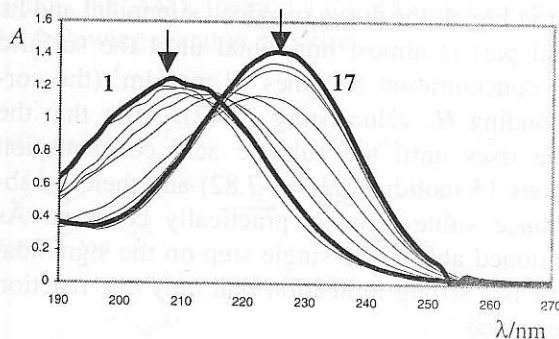
Fig. 1. Ultraviolet spectra of glutamic acid ( c = 1.09 \cdot 10^{-4} mol/dm 3 ) in sulfuric acid media (from c = 1 mol/dm 3 , spectrum 1, to c = 17 mol/dm 3 , spectrum 17)
