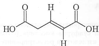
cis -glutaconic acid
