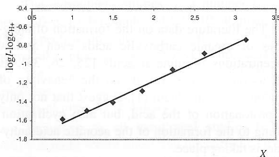
Fig. 8. Dependence of \log I - \log c_{\text{H}^+} on X for glutaconic acid ( c = 1.01 \cdot 10^{-4} \text{ mol/dm}^3 ) in sulfuric acid media (from c = 1 \text{ mol/dm}^3 to c = 17 \text{ mol/dm}^3 )
