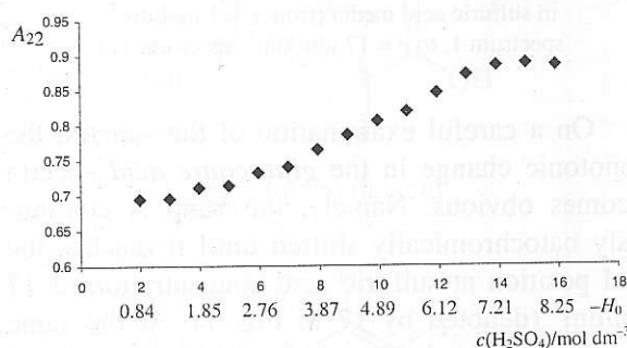
Fig. 4. Absorbance values ( \lambda = 226 \text{ nm} ) for glutamic acid as a function of the sulfuric acid concentration
