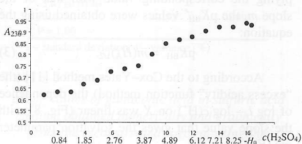
Fig. 5. Absorbance values ( \lambda = 236 nm) for aconitic acid as a function of the sulfuric acid concentration
