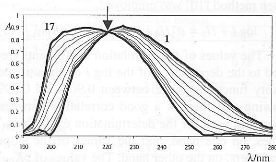
Fig. 6. Reconstructed ultraviolet spectra of aconitic acid ( c = 1.01 \cdot 10^{-4} mol/dm 3 ) in sulfuric acid media (from c = 1 mol/dm 3 , spectrum 1, to c = 17 mol/dm 3 , spectrum 17)
