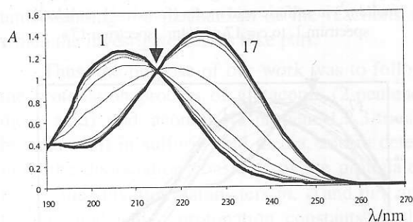
Fig. 3. Reconstructed ultraviolet spectra of glutamic acid ( c = 1.09 \cdot 10^{-4} \text{ mol/dm}^3 ) in sulfuric acid media (from 1 \text{ mol/dm}^3 , spectrum 1, to c = 17 \text{ mol/dm}^3 , spectrum 17)
