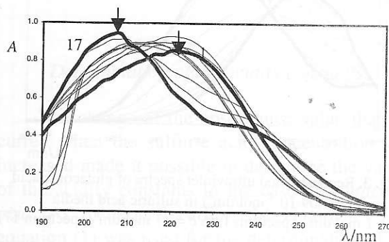
Fig. 2. Ultraviolet spectra of aconitic acid ( c = 1.01 \cdot 10^{-4} mol/dm 3 ) in sulfuric acid media (from c = 1 mol/dm 3 , spectrum 1, to c = 17 mol/dm 3 , spectrum 17)
