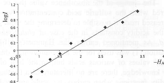
Fig. 7. Dependence of the ionization ratio, I = c_{\text{BH}^+}/c_{\text{B}} , of glutaconic acid ( c = 1.01 \cdot 10^{-4} \text{ mol/dm}^3 ) on the amide acidity function ( H_A )
