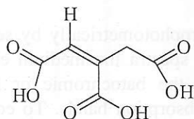
cis -aconitic acid ( E )
