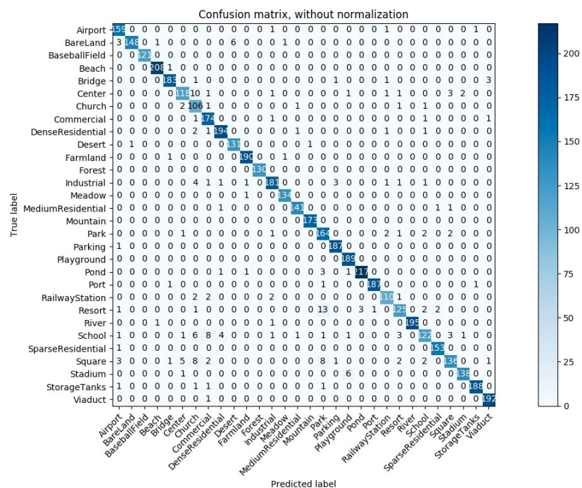
Figure 9. Confusion matrix of the proposed method with a 50%/50% train/test ratio of AID data set for ResNet50, linear learning rate decay, and softmax classifier.
