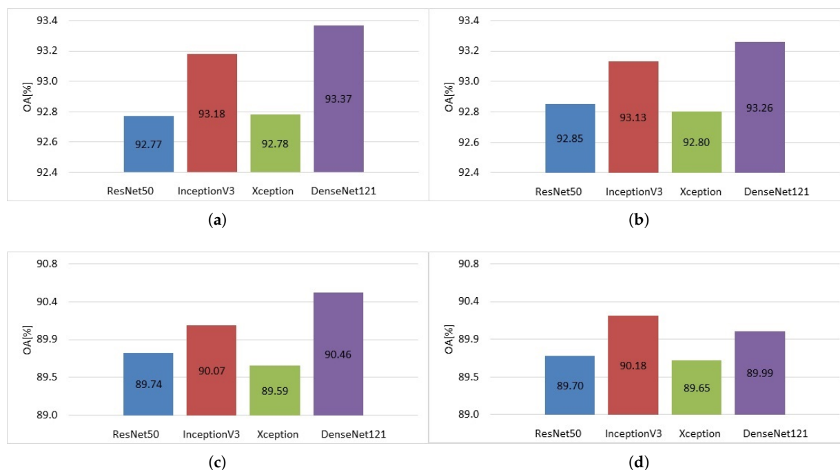
Figure 13. Overall Accuracy over five runs for NWPU-RESISC45 data set with linear SVM classifier and (a) 20% /80% train/test split ratio, linear decay scheduler; (b) 20% /80% train/test split ratio, cyclical learning rates; (c) 10% /90% train/test split ratio, linear decay scheduler; (d) 10% /90% train/test split ratio, cyclical learning rates.
