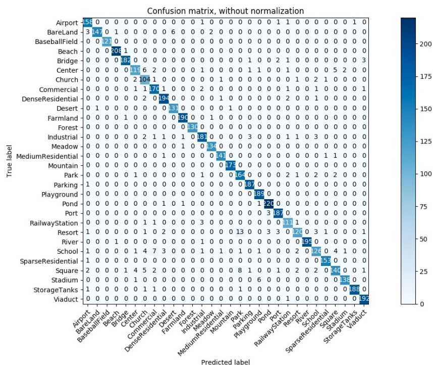
Figure 10. Confusion matrix of the proposed method with a 50%/50% train/test ratio of AID data set for ResNet50, linear learning rate decay, and a linear SVM classifier.
