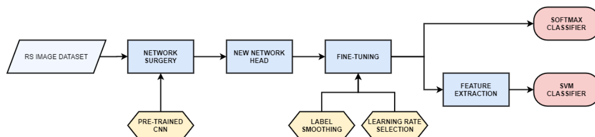
Figure 1. Flowchart of the proposed method.
