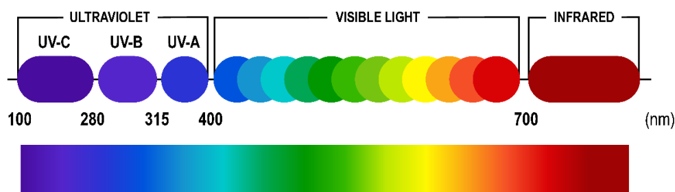
Figure 1: The solar spectrum.
