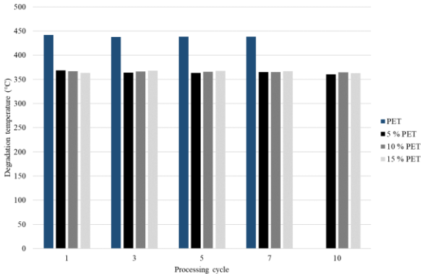
Figure 2. Degradation temperatures determined by TGA
