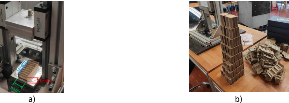
Figure 2: Experimental determination of honeycomb cushioning characteristics; a) Experimental test rig, b) Specimen before and after testing.
