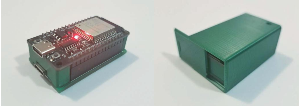
Figure 1: Final assembly of the packaging motion sensor prototype
