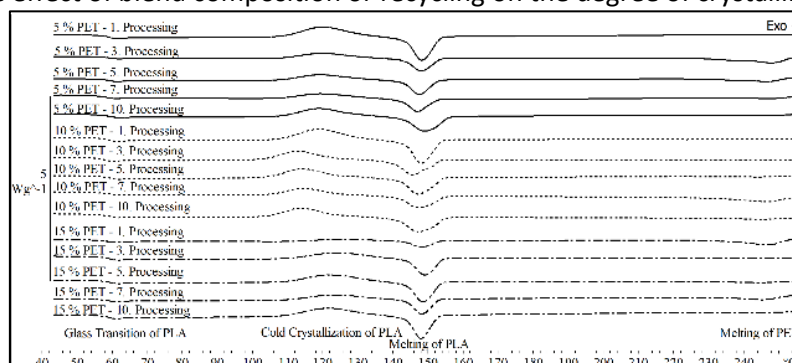
Figure 1. DSC thermograms of second heating recorded for blends
