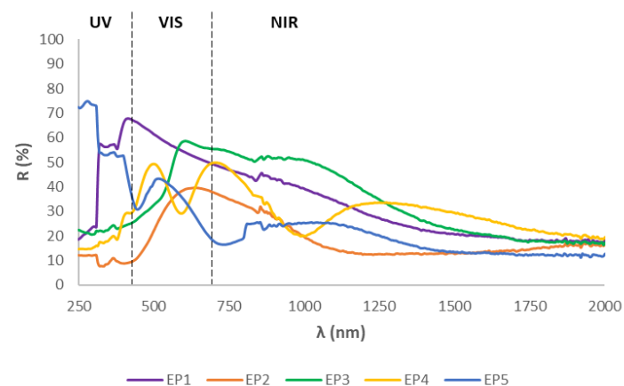
Figure 6: Reflectance spectra of printed pigments on OPP film in the UV-VIS-NIR regions.
