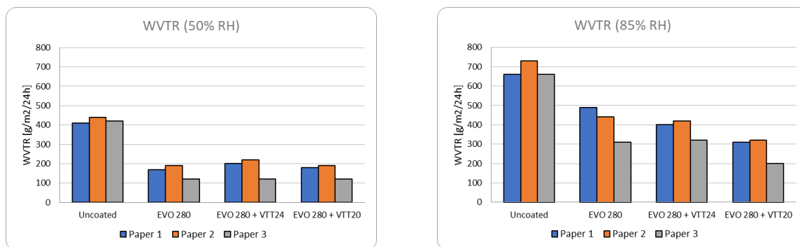
Figure 2: WVTR of uncoated and coated paper samples at 50% RH and 85% RH.
