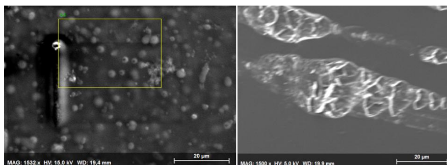
Figure 2: SEM micrographs of gelatin–zein (left) and gelatin–psyllium (right) films at 1500x magnification
