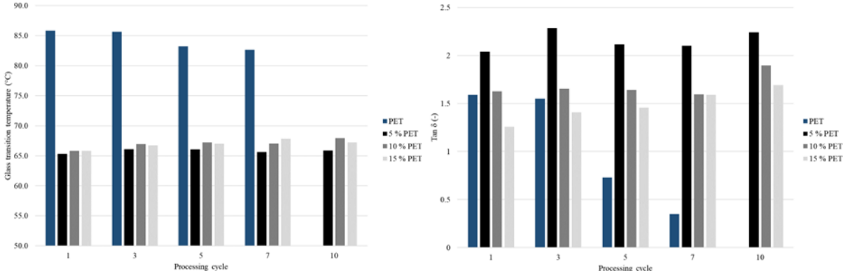
Figure 3. Glass transitions (left) and loss factor values at peak (right) determined by DMA
