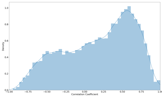
Fig. 1. Distribution of coefficients in the cryptocurrency correlation matrix.
