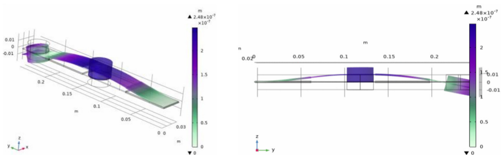
Fig. 12. Piezoelectric transducer placed on a cantilever with additional masses m_1 = 94 g and m_2 = 94 g for resonant frequency 51.1 Hz
