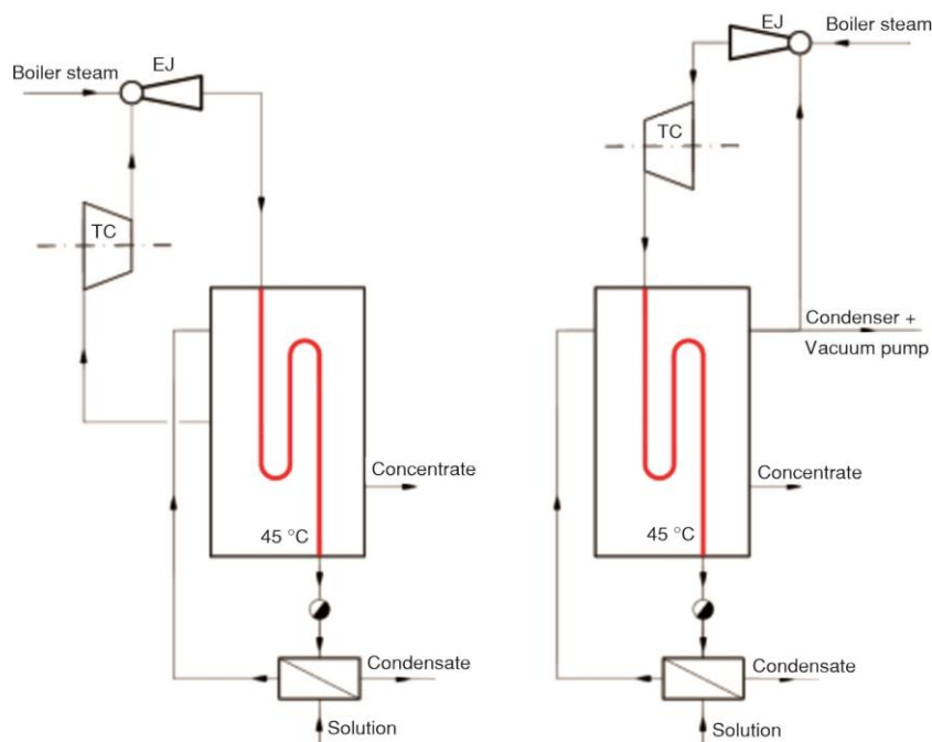
Figure 8. Combined concentrator system with turbocompressor and ejector
