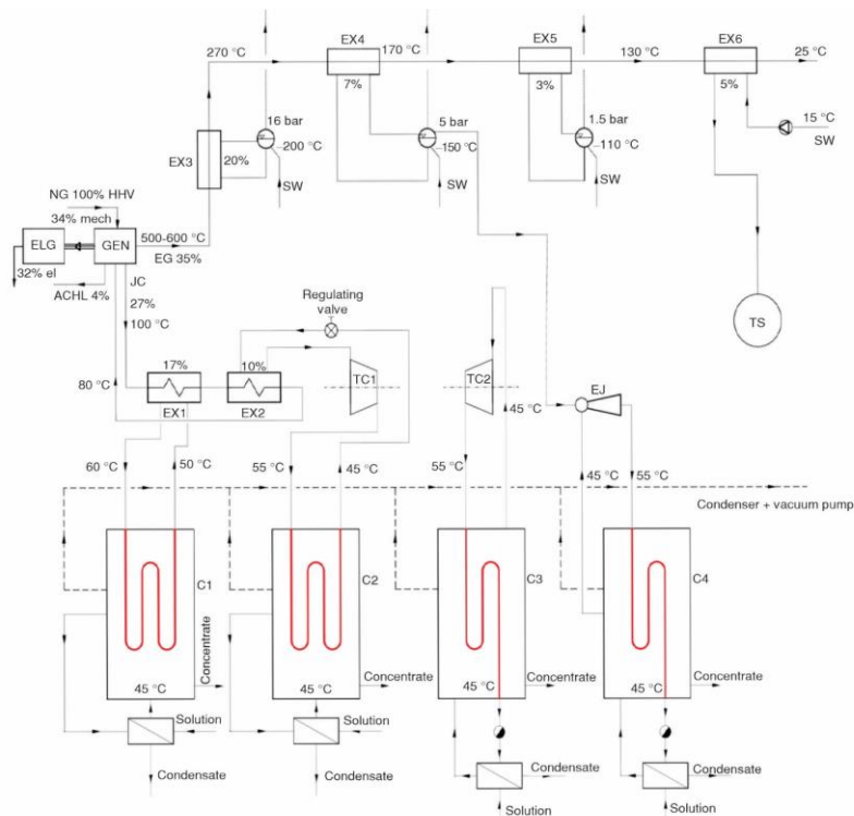
Figure 9. Polygeneration for production of electricity, technological water vapor and technological hot water with turbocompressor and ejector thermocompression
