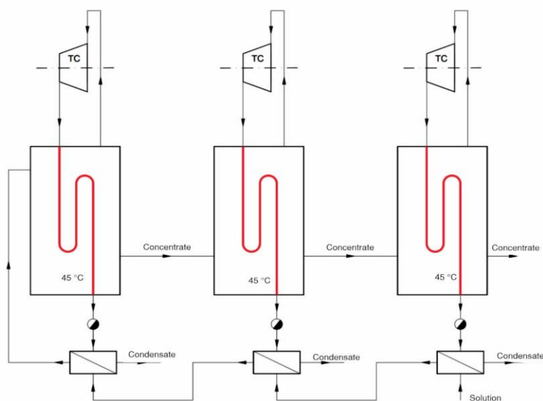
Figure 3. Multistage concentrator system with three turbocompressor units
