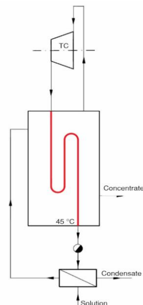
Figure 2. Single stage turbocompressor thermocompression concentrator
