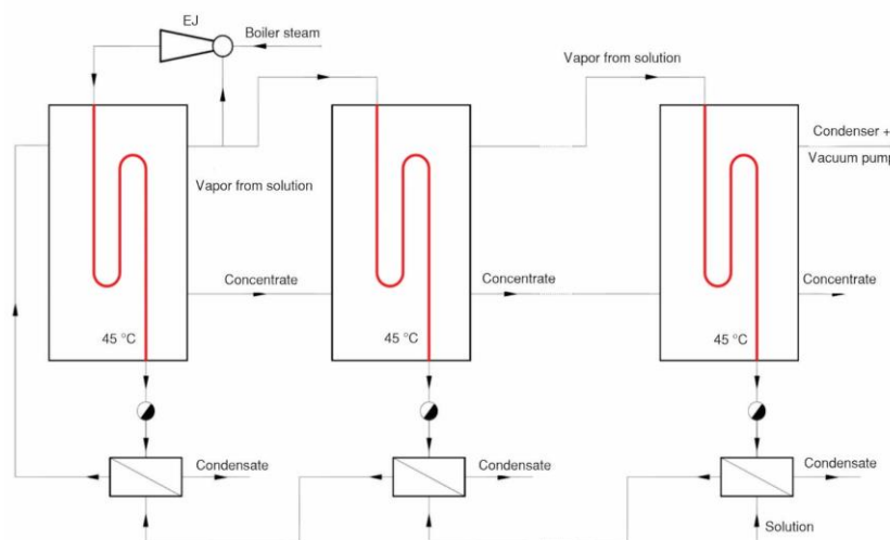
Figure 7. Multistage concentrator system with ejector thermocompression
