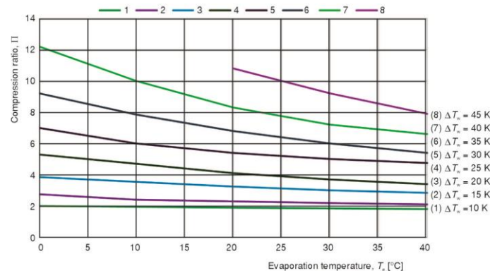
Figure 1 Dependence of R718 pressure ratio ( \Pi ) on evaporating temperature, T_e , for different values of the temperature lift, \Delta T_w
