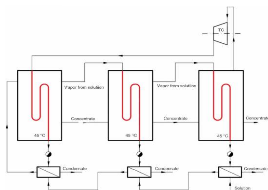
Figure 4. Multistage concentrator system with one high pressure turbocompressor unit
