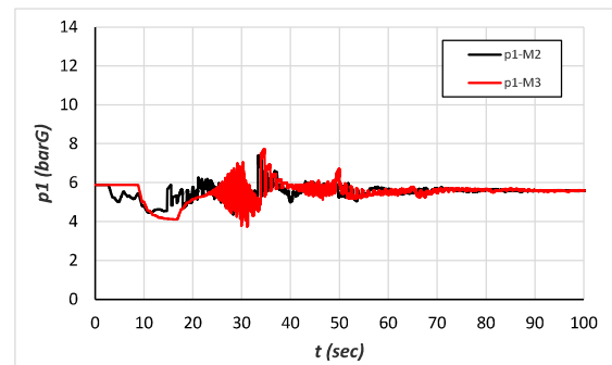
b) pipeline of different wall material at parallel branches (M2 & M3)
