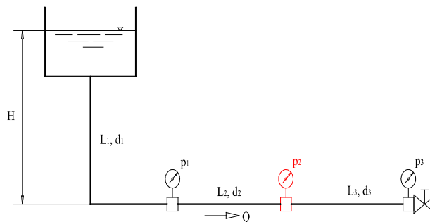
Figure 4. Pipeline with serial connection of branches (Case 4)
