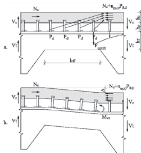
Figure 2. Vierendeel bending and Vierendeel resistance moment due to composite action.
