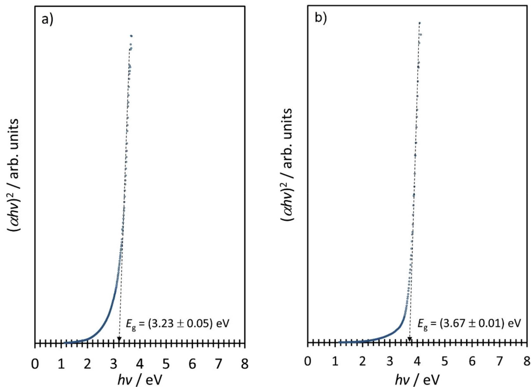
Fig. 14 (\alpha hv)^2 vs. hv dependency of (a) NiO-a and (b) NiO-c NPs obtained through the thermal treatment of the \beta -Ni(OH) 2 and Ni 3 (OH) 4 (NO 3 ) 2 intermediates, respectively.
