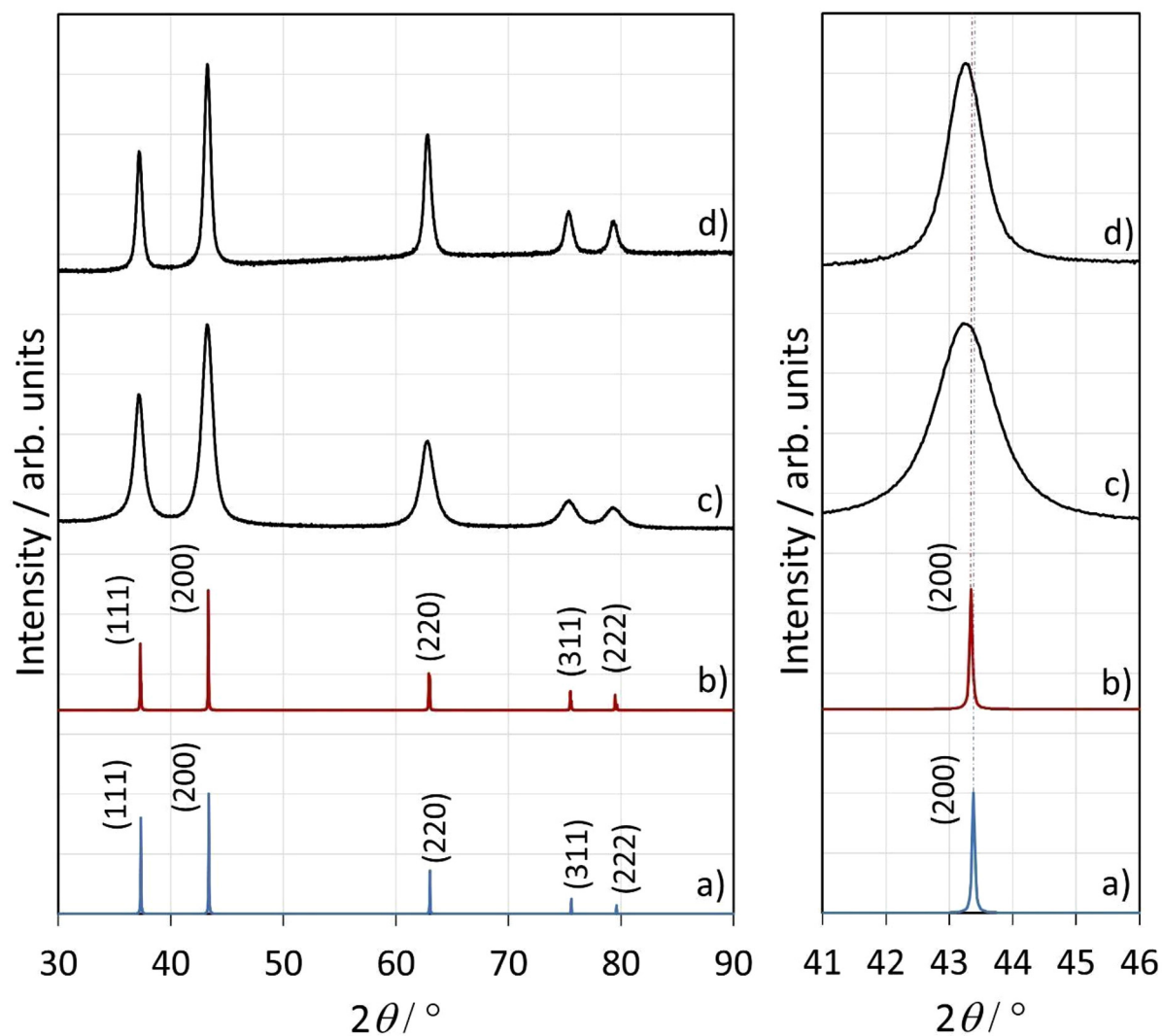
Fig. 5 The left panel represents the XRD patterns of reference (a) cubic \text{NiO}^{\text{71}} and (b) non-stoichiometric \text{NiO}_{x}^{\text{70,71}} and NiO obtained using ammonia (c) and carbamide (d) precursors. The right panel shows the (200) reference peaks in comparison to the experimental peaks of NiO obtained by both precursors.
