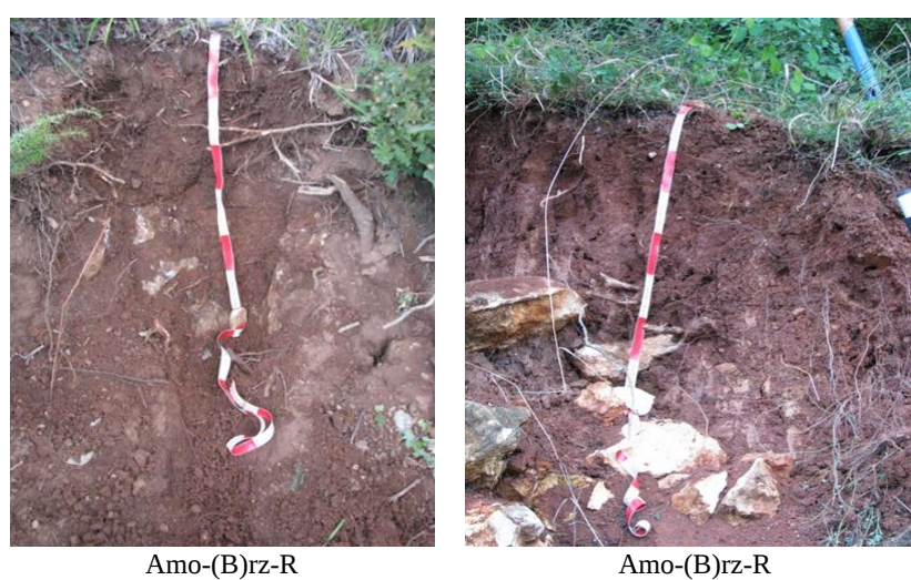
Figure 5. Terra Rossa
