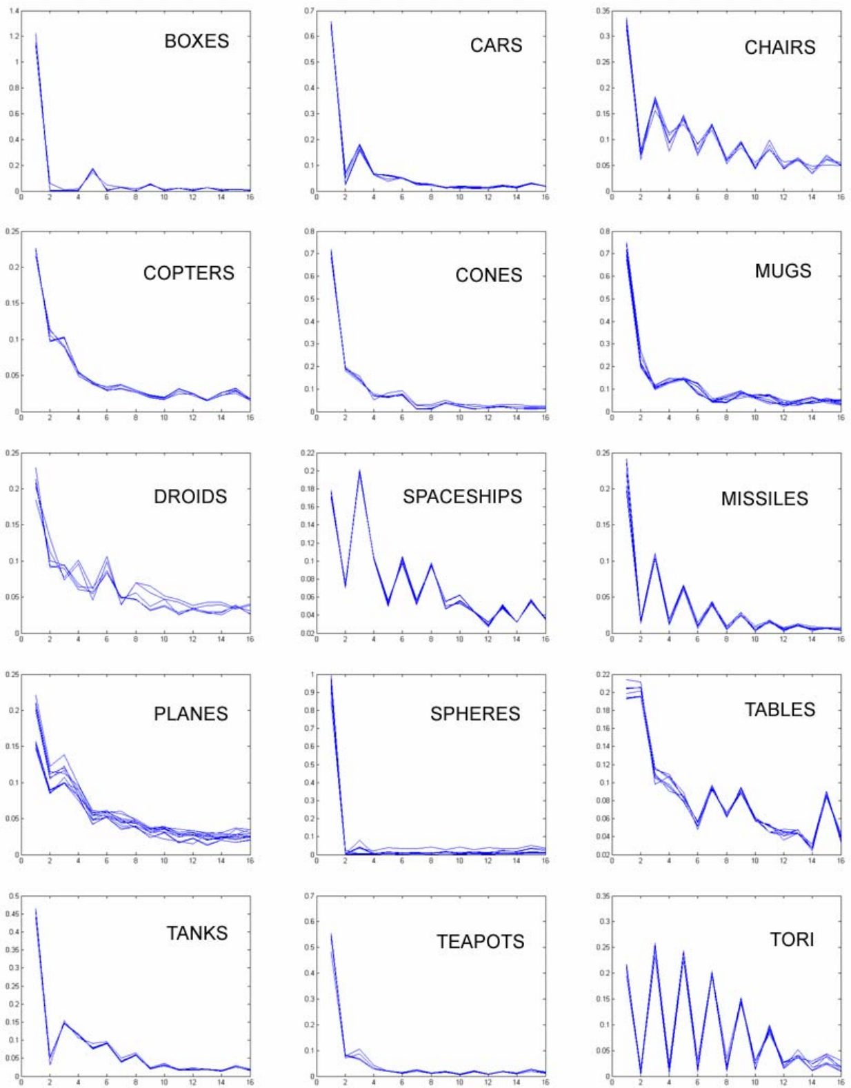
Fig. 5. Robustness test for the descriptor based on spherical harmonics.
