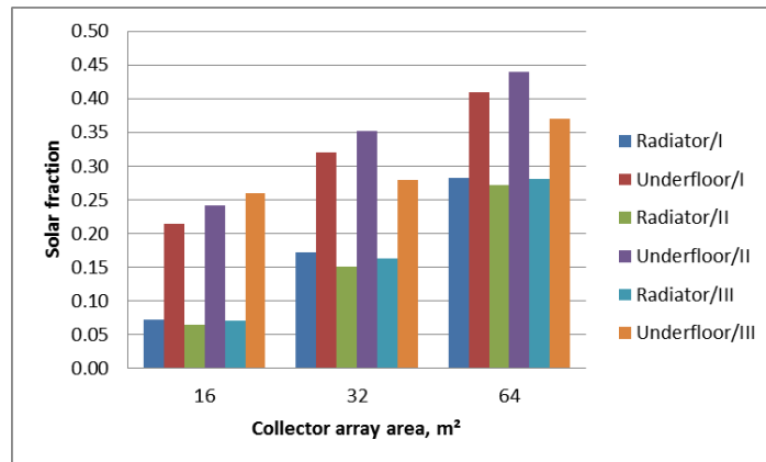
Figure 4. Solar fraction for heating with storage tank 1500l regard of collector array area building type
