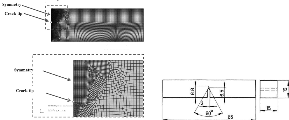
Fig. 1. Geometry and mesh configuration of center-cracked SENB specimen
