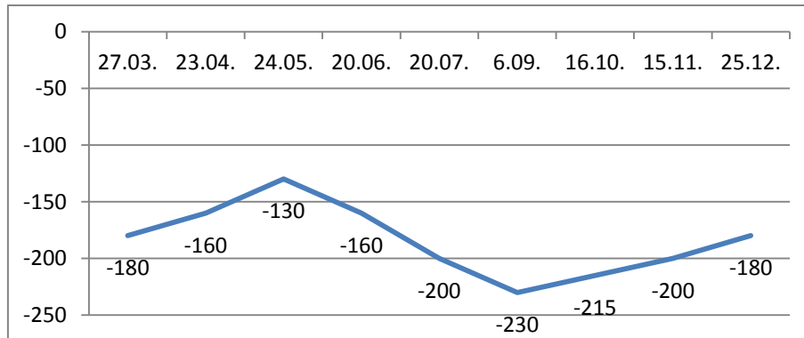
Figure 1 The level of groundwater in profile P1
