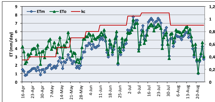
Figure 2. Daily evapotranspiration and crop coefficient of maize
