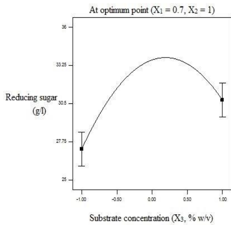
Fig 4.3 Effect of substrate concentration on reducing sugar at optimum point Fig 4.4 Effect of enzyme loading ratio and time on reducing sugar at optimum point
