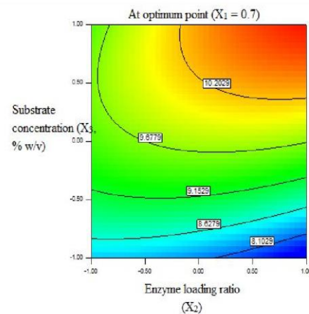
Fig 7 Effect of enzyme loading ratio and substrate concentration on lignin at optimum
