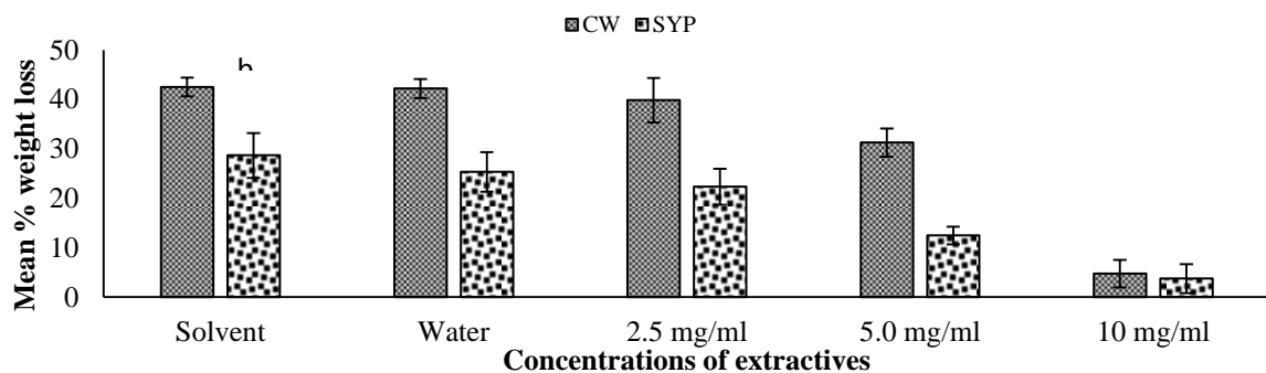
Fig. 6. Mean percentage weight loss of SYP and CW blocks vacuum impregnated with P. roxburghii extractives after termites feeding.
