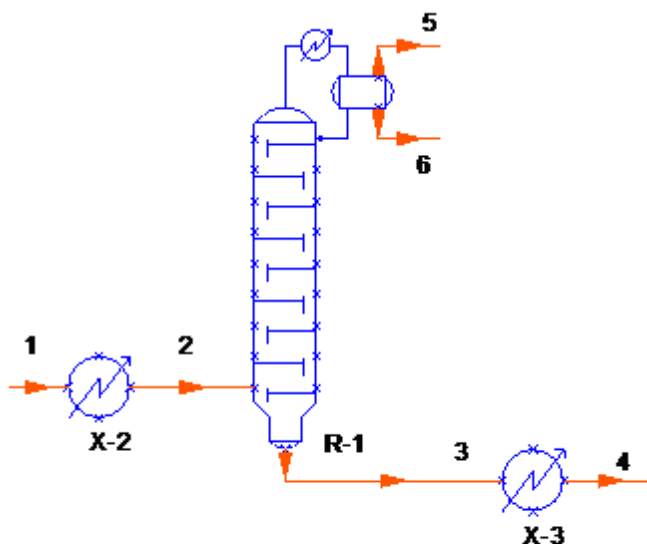
Figure 3. The simulation scheme in Design II, for preflash unit in crude oil distillation process
