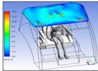
Figure 9. Front vents
