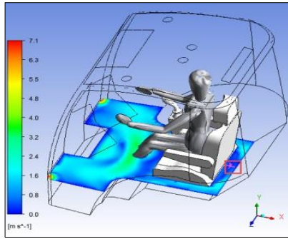
Figure 6. Behind seat
