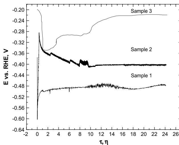
Fig. 7 – Long-term galvanostatic test of the studied electrode materials in EasyTest Cell at 0.3 \text{ A cm}^{-2} for 24 h.
