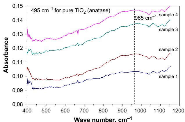
Fig. 4 – Infrared spectra of \text{TiO}_2 originated from the studied electrocatalysts.
