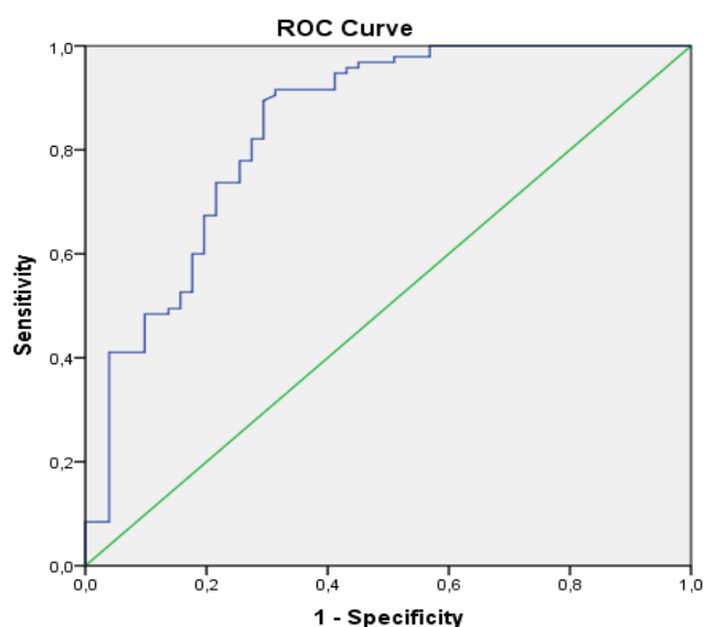
Fig. 2. ROC area
