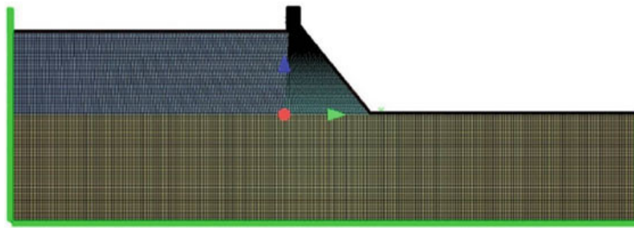
Fig. 6 Fine finite element mesh ( N = 54440 ), applied for Case C (green lines at model edges represent the dampers)
