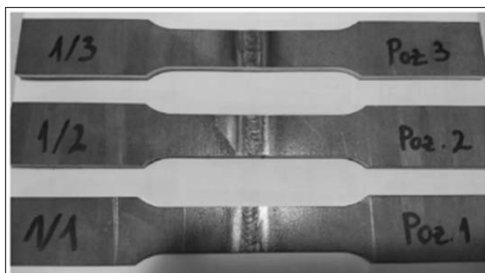
Figure 6. Tensile testing specimens
