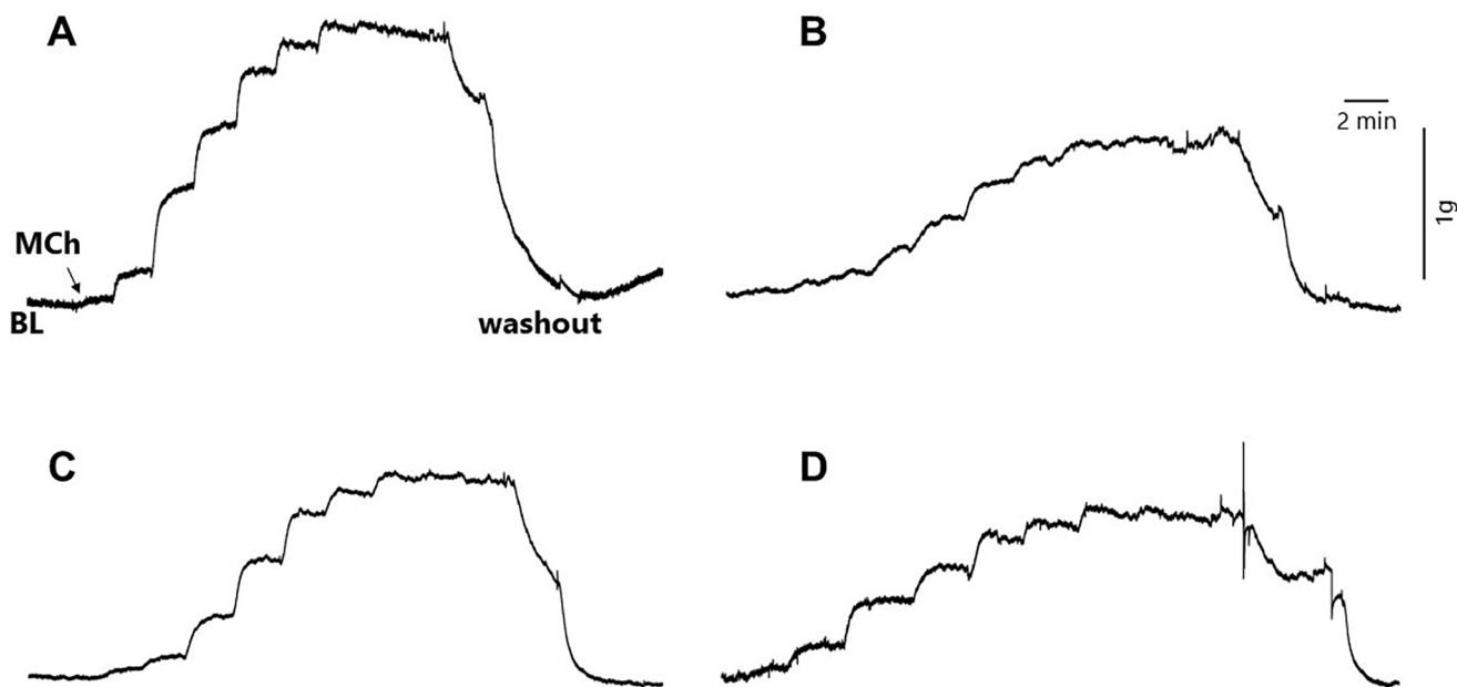
Figure 2. Tracings of representative recordings showing the methacholine-induced TSM contraction: (a) H-control, (b) H-quercetin, (c) AA control, and (d) AA-quercetin. MCh: methacholine; BL: baseline.
