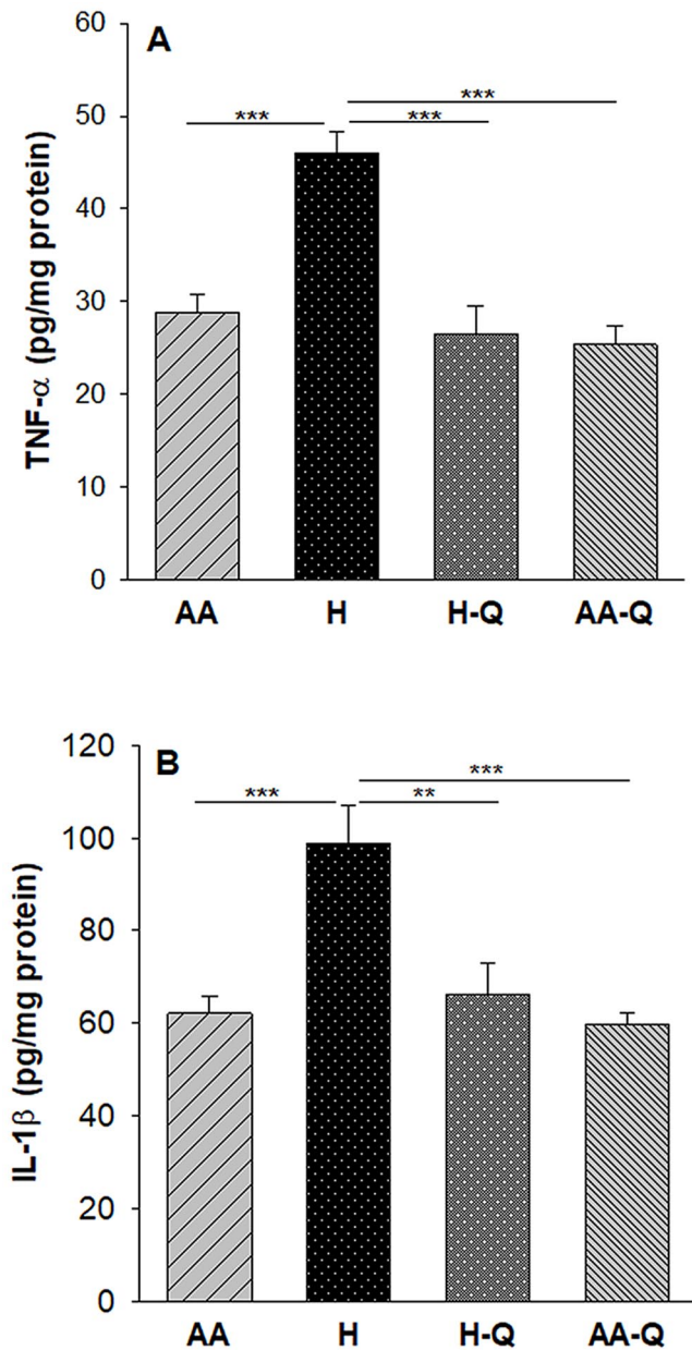
Figure 6. Effect of quercetin on proinflammatory cytokines in lung tissue of rat pups: (a) TNF- \alpha level in lung tissue of rat pups exposed to hyperoxia or AA ( n=6 , each condition) and (b) IL-1 \beta level in lung tissue of rat pups exposed to hyperoxia or AA ( n=7 , each condition). ** P < 0.01 ; *** P < 0.001 . H: hyperoxia; AA: ambient air; H-Q: hyperoxia + quercetin; AA-Q: ambient air + quercetin. Data reported as mean \pm SEM.
