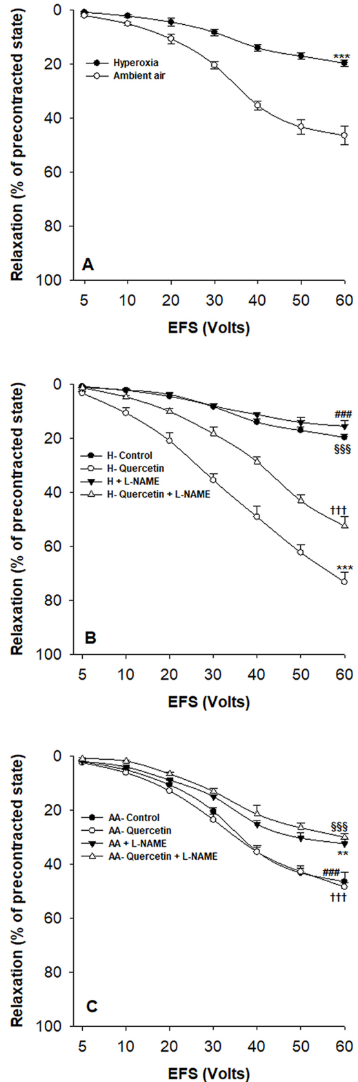
Figure 4. Effect of in vitro quercetin supplementation and NOS inhibition on EFS-induced relaxation of TSM of rat pups: (a) relaxant responses of TSM in hyperoxic and AA control groups (***P<0.001; n=9 and n=6, respectively) and (b) relaxant responses of TSM of hyperoxia-exposed rat pups in the absence or presence of quercetin (100 μM) and/or L-NAME (100 μM) (n=9, each condition; ***P<0.001 – H-quercetin versus H-control/H+ L-NAME; †††P<0.001 – H-quercetin + L-NAME versus H-quercetin; §§§P<0.001 – H-control versus H-quercetin + L-NAME; ###P<0.001 – H+ L-NAME versus H-quercetin + L-NAME). (c) Relaxant responses in AA groups in the absence or presence of quercetin (100 μM) and/or L-NAME (100 μM) (n=6, each condition; **P<0.01 – AA + L-NAME versus AA control; §§§P<0.001 – AA-quercetin + L-NAME versus AA control; ###P<0.001 – AA-quercetin versus AA + L-NAME; †††P<0.001 – H-quercetin versus AA-quercetin + L-NAME. H: hyperoxia; AA: ambient air. Values are mean ± SEM.
