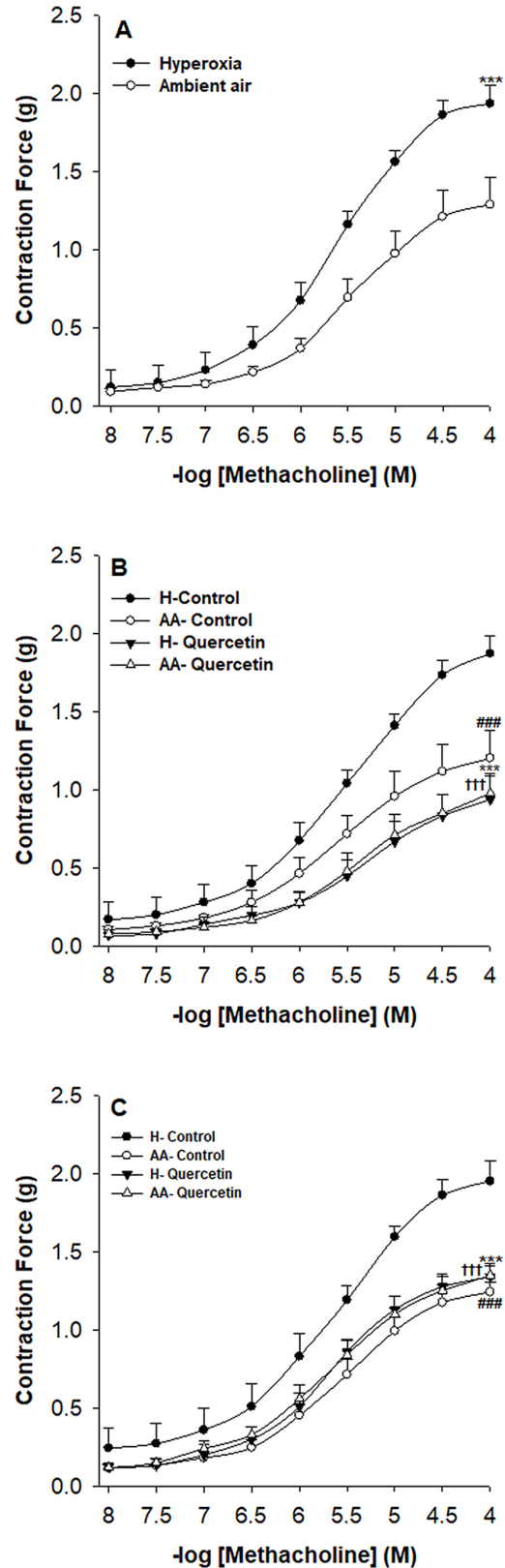
Figure 1. The effect of in vitro and in vivo quercetin supplementation on methacholine-induced contraction of TSM of rat pups: (a) contractile responses of TSM in hyperoxic and AA control groups ( ***P < 0.001 ; n = 10 , each condition), (b) contractile responses of TSM obtained from hyperoxic and AA groups in the absence or presence of quercetin supplemented in vitro (100 \mu M) ( n = 10 , each condition), and (c) contractile responses of TSM obtained from hyperoxic and AA groups supplemented with quercetin in vivo (10 mg \cdot kg ^{-1} \cdot day ^{-1} ) ( n = 7 , each condition). ( ***P < 0.001 – H-quercetin versus H-control; †††P < 0.001 – AA-quercetin versus H-control; ###P < 0.001 – AA control versus H-control). H: hyperoxia; AA: ambient air. Values are mean \pm SEM.
