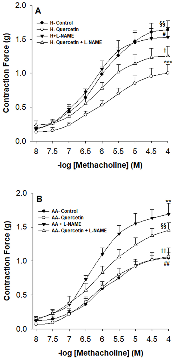
Figure 3. Effect of NOS blockage on quercetin-reversed airway hyperreactivity: (a) contractile responses of TSM in hyperoxia-exposed rat pups in the absence or presence of L-NAME (100 μM) and/or quercetin (100 μM) (n=11, each condition; ***P<0.001 – H-quercetin versus H+ L-NAME/H-control; †P<0.05 – H-quercetin + L-NAME versus H-quercetin; §§P<0.01 – H-control versus H-quercetin + L-NAME; *P<0.05 – H+ L-NAME versus H-quercetin + L-NAME). (b) Contractile responses of TSM of AA-exposed rat pups in the absence or presence of L-NAME (100 μM) and/or quercetin (100 μM) (n=6, each condition; **P<0.01 – AA + L-NAME versus AA control; §§P<0.01 – AA-quercetin + L-NAME versus AA control; ##P<0.01 – AA-quercetin versus AA + L-NAME; †P<0.05 – AA-quercetin versus AA-quercetin + L-NAME. H: hyperoxia; AA: ambient air. Values are mean ± SEM.
