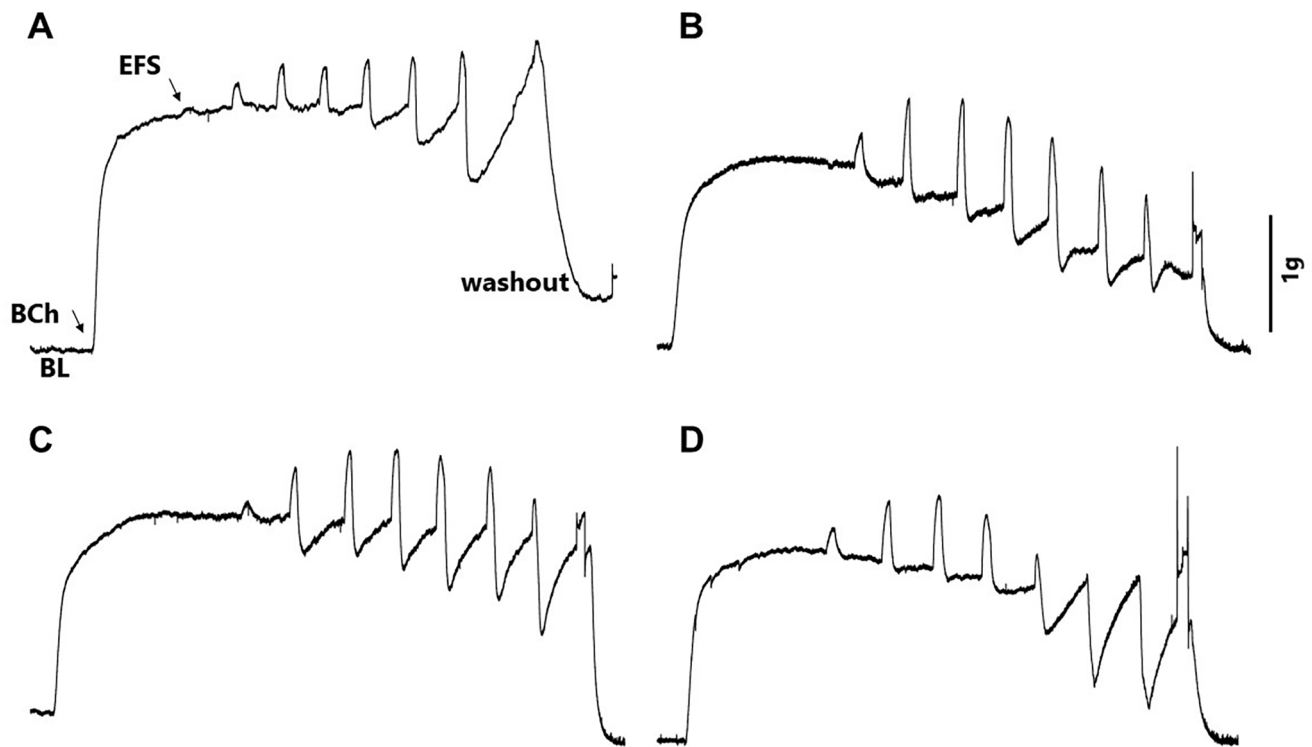
Figure 5. Tracings of representative recordings showing the EFS-induced relaxation of precontracted TSM: (a) H-control, (b) H-quercetin, (c) AA control, and (d) AA-quercetin. BCh: bethanechol, BL: baseline.
