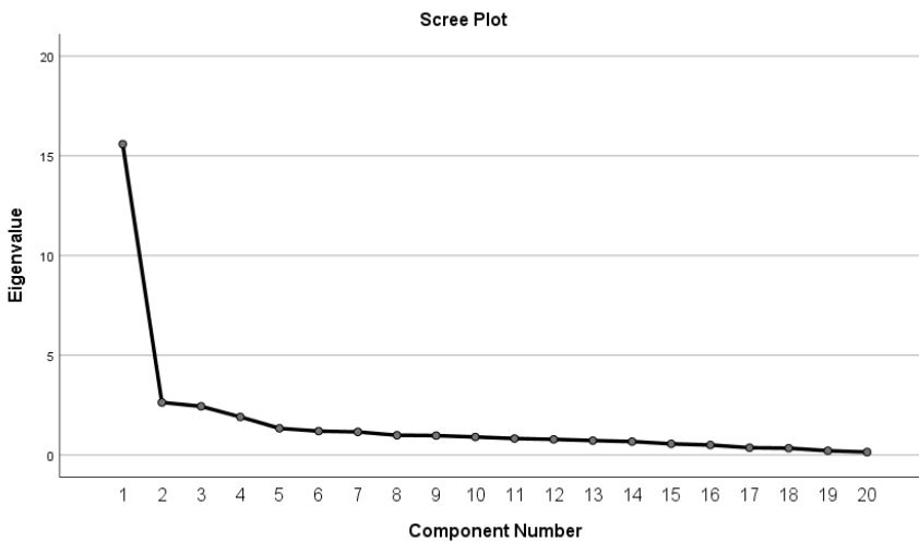
Figure 1. Scree Plot
