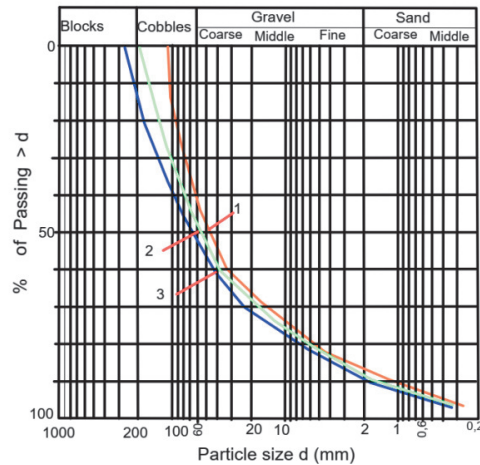
Figure 3. Granulometric curves for rockfill (1) and cases with VBP=15% (2) and VBP=35% (3).
