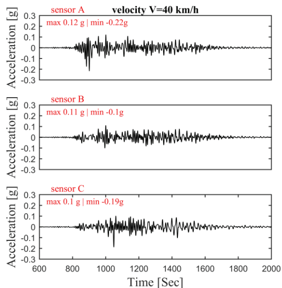
Figure 8. Time history plot of vertical accelerations and maximal amplitudes for velocity 40km/h for Bridge B05
