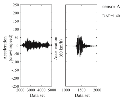
Figure 10. Signals for DAF estimation, velocity 60km/h, Bridge B15
