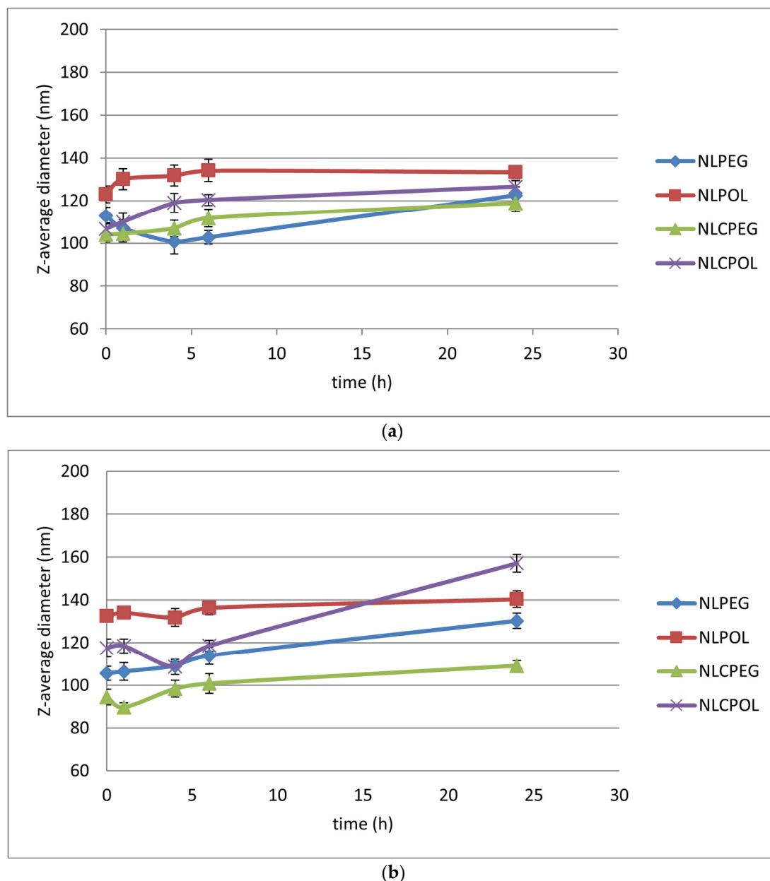
Figure 2. Mean particle size of NL and NLC samples incubated in a period of 24 h in: (a) phosphate buffer pH 7.4; and (b) human plasma.
