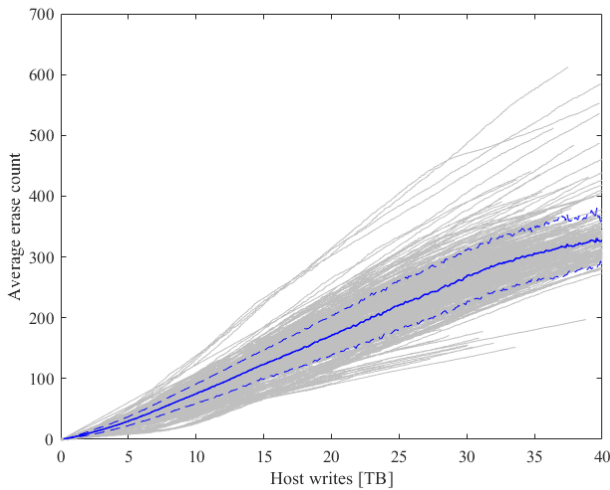
Fig. 3. Average erase count for ZA250CM10002 SSD
