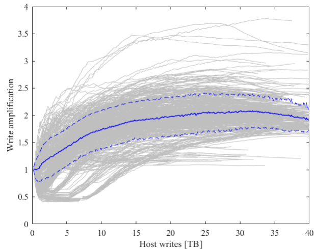
Fig. 5. Write amplification for ZA250CM10002 SSD
