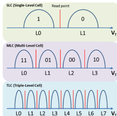
Fig. 1. FLASH cell technologies
