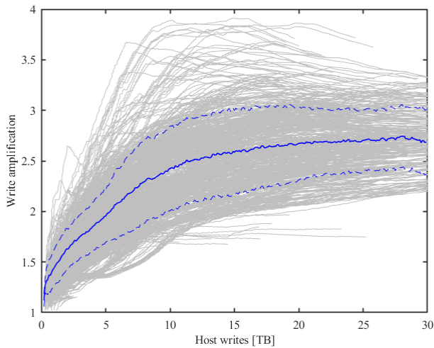
Fig. 6. Write amplification for ZA250CM10003 SSD
