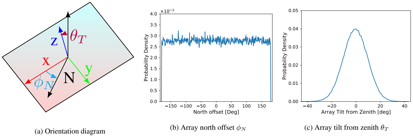
Figure 4: Array orientation
