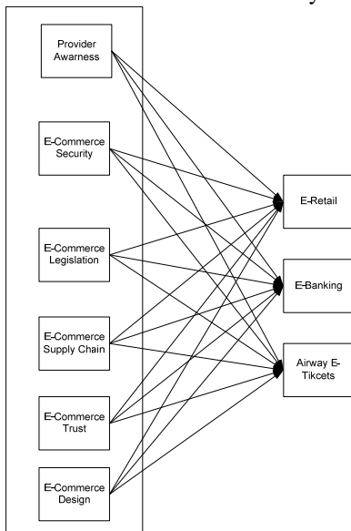
Fig. 8 Research Model
