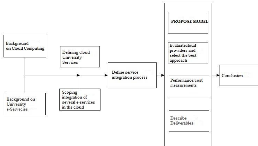
Fig.5. Research Approach
