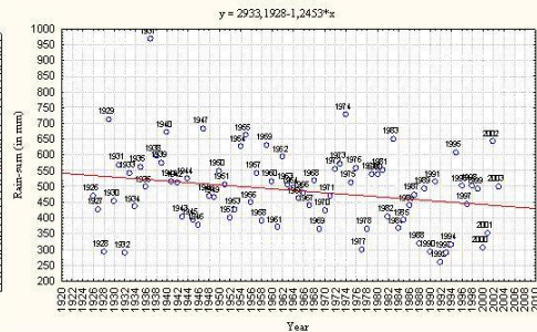
Observed values and their regression line of average annual rain-sums in Skopje for 1925-2003
