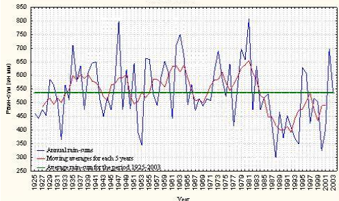
Rain-sums and moving averages (for 5 years) in Prilep for 1925-2003
