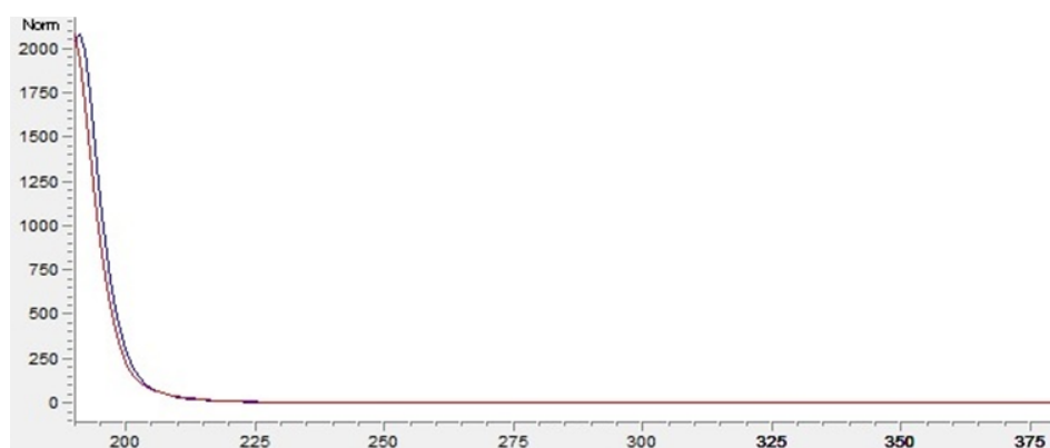
Figure 6. Overlaid spectra of peak 1 from all samples
