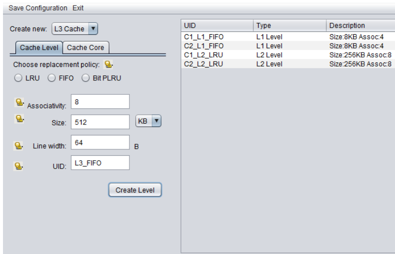
Fig. 3: Overview of design mode of EDUCache simulator - Creating L3 cache instance
