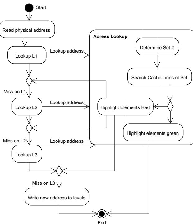
Fig. 8: Activity diagram of the steps that update the visual representation
