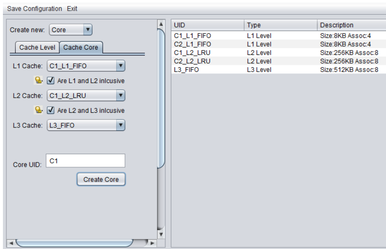
Fig. 4: Overview of design mode of EDUCache simulator - Creating a CPU core
