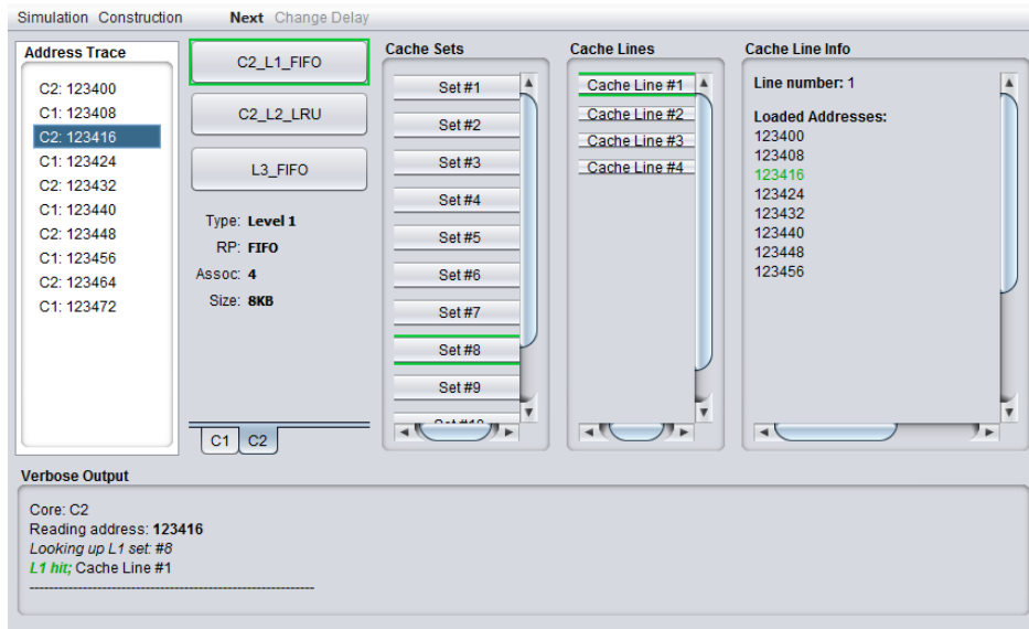
Fig. 5: Overview of Simulation mode - hit in L1 level of core C2, set #8, line #1, address 123416
