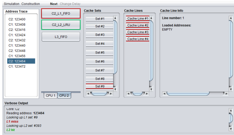
Fig. 9: Overview of simulation mode of EDUCache simulator, L1 miss and L2 hit while reading the address 123464
