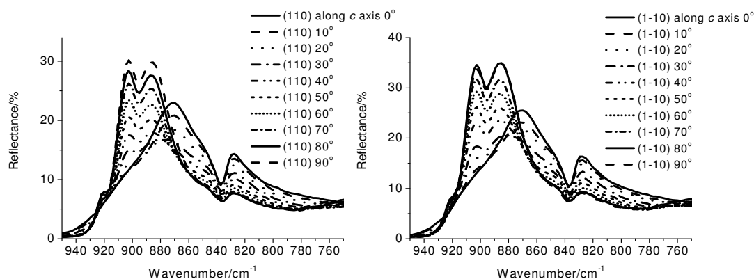
Fig. 3. Polarized reflectance spectra recorded from the (110) and (1-10) planes in a KNiSeH single crystal. The crystal was rotated about the normal to the planes counterclockwise and clockwise, respectively, with a step of 10^\circ , starting with polarization along the c direction. Spectra for each polarization angle recorded from different plane are the same. Due to different polishing qualities of the crystal faces, the reflectance from the two planes differs slightly.
