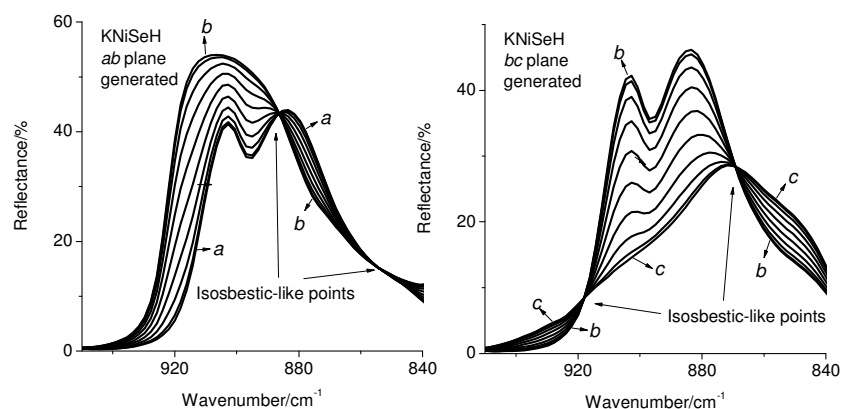
Fig. 6. Generated polarized IR reflectance spectra for KNiSeH single crystal planes ab , (001) and bc , (100), using eq. (1). Recorded spectra with polarization along the a and b axes for (001), while spectra with polarization along the b and c axes for (100) were needed for the generation of the other spectra. ILP instead of ILR appears here. The spectra are practically identical to the originally measured in Figure 5.
