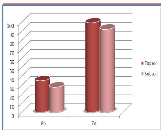
Fig. 8. Average values of the elements of Factor 2 in surface and subsurface soil
