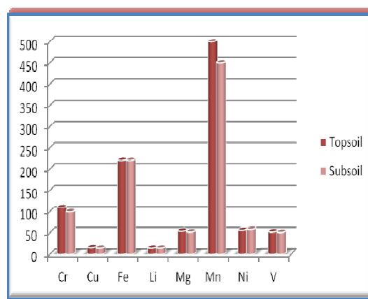
Fig. 6. Average contents of the elements of Factor 1 in surface and subsurface soil
