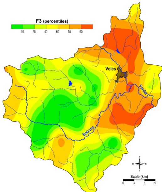
Fig. 11. Spatial distribution of factor values of Factor 3 (Al, Ca)
