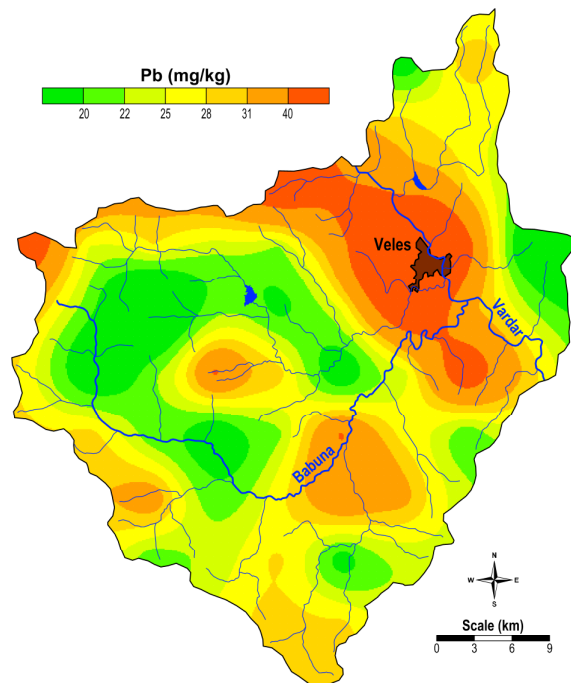
Fig. 9. Spatial distribution map of Pb
