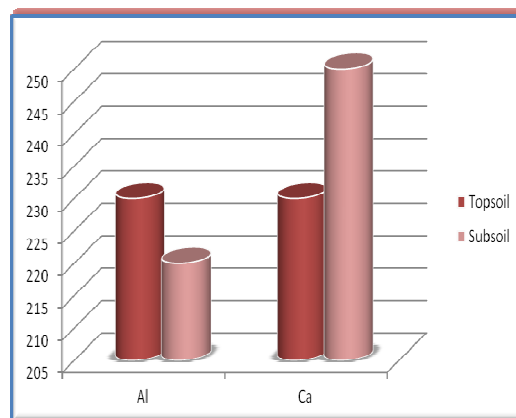
Fig. 12. Average values of the elements of Factor 3 in surface and subsurface soil
