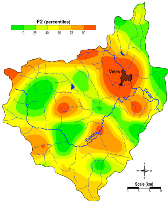
Fig. 7. Spatial distribution of factor values of Factor 2 (Pb, Zn)
