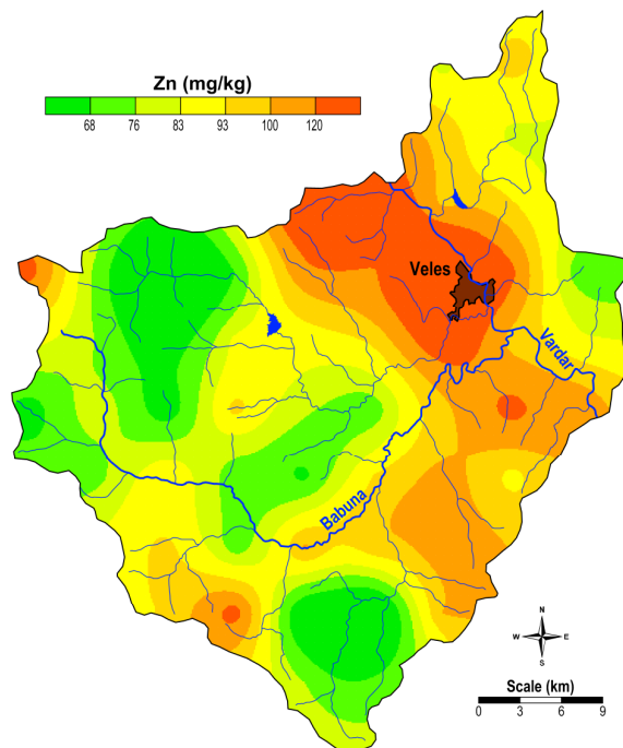
Fig. 10. Spatial distribution map of Zn
