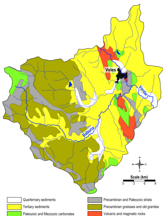
Fig. 2. Geological map of the studied area
