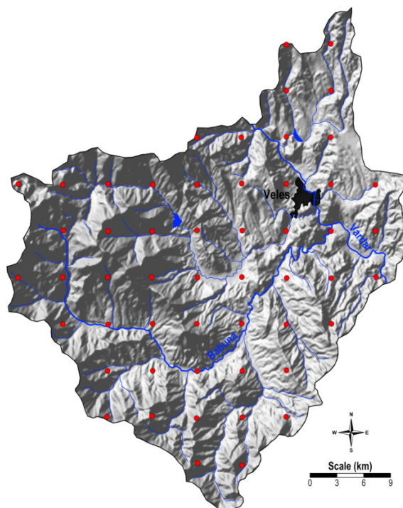
Fig. 3. Sampling location map
