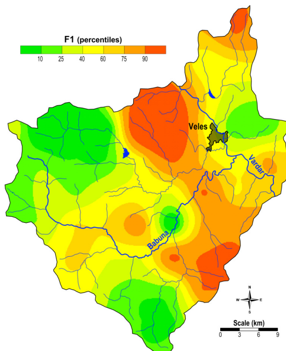
Fig. 5. Spatial distribution of factor values of Factor 1 (Cr, Cu, Fe, Li, Mg, Mn, Ni and V)
