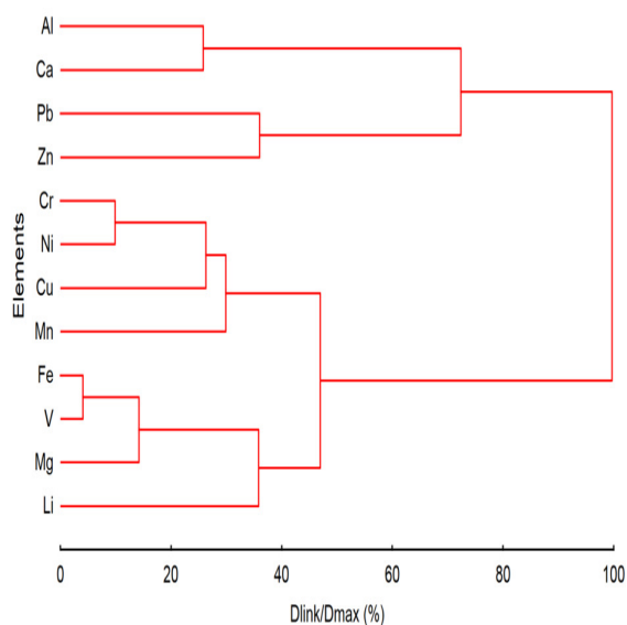
Fig. 4. Dendrogram from cluster analysis
