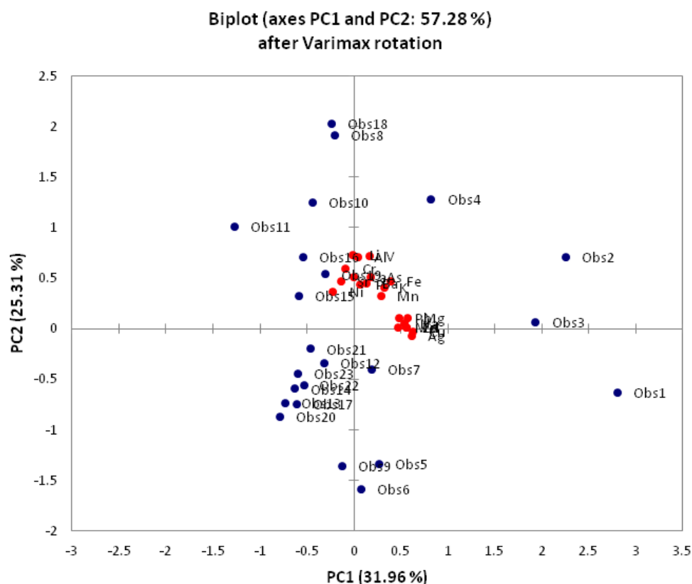
Fig. 6. Biplot for moss species vs. elements contents
