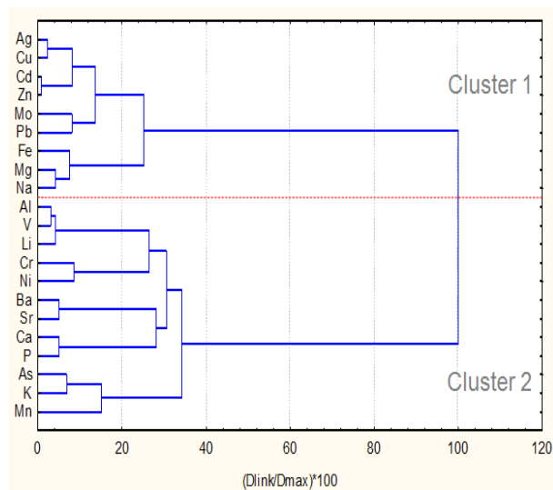
Fig. 7. Clusters for elements associations (Tree diagram, Vard's method, 1 – Pearson r )
