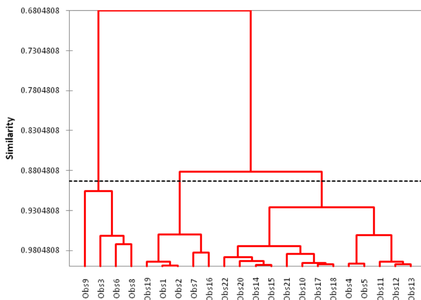
Fig. 8. Cluster analyses for observations (moss species locations)
