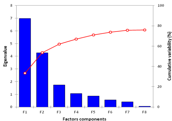
Fig. 3. Scree plot for Eigene values
