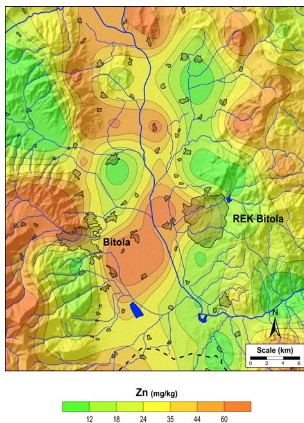
Fig. 3. Spatial distribution of zinc
