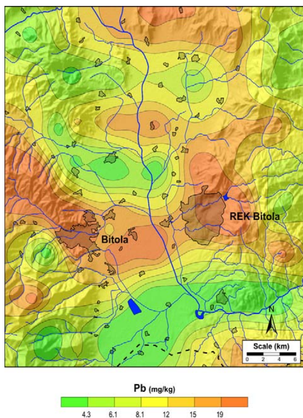
Fig. 2. Spatial distribution of lead
