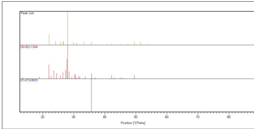
Figure 3. XRD patterns of glass-ceramics of NFA sintered at 1050 °C/60', Phase 1: Calcium Aluminum Silicate 00-052-1344; Phase 2: Iron oxide (III) reference ICSD. 01-073-0603
