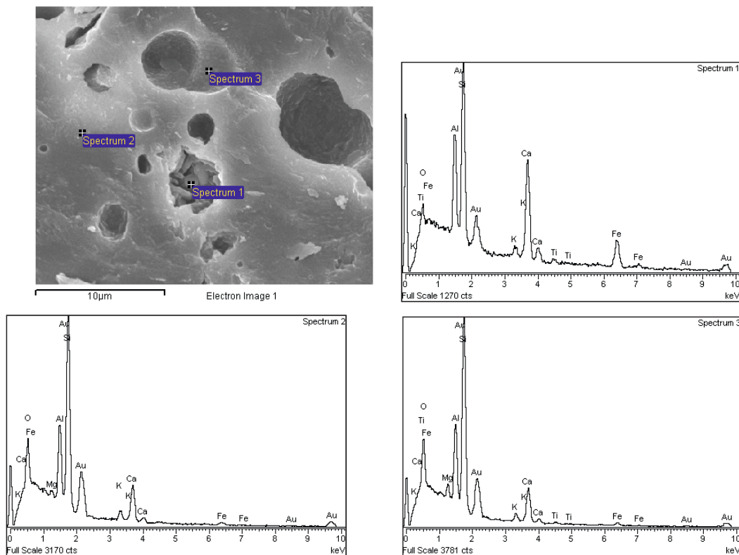
Figure 8. EDS analysis of glass-ceramic sample from NFA, sintered at 1050/60 min
