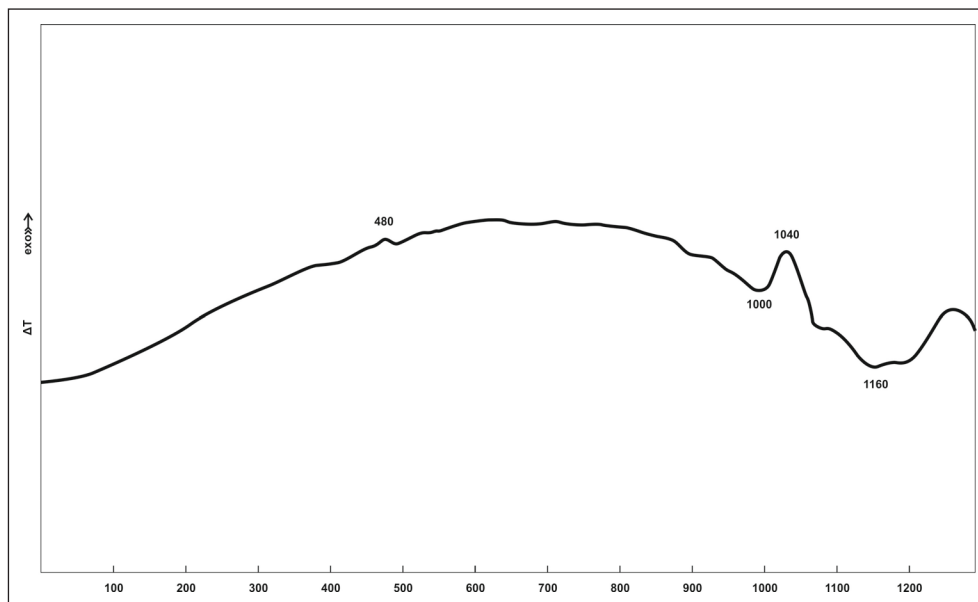
Figure 2. DTA curve of glass sample at heating rate of 10 °C/min
