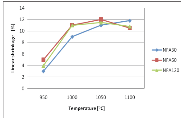
Figure 5. Linear shrinkage of glass-ceramics after exposure on defined temperature treatments
