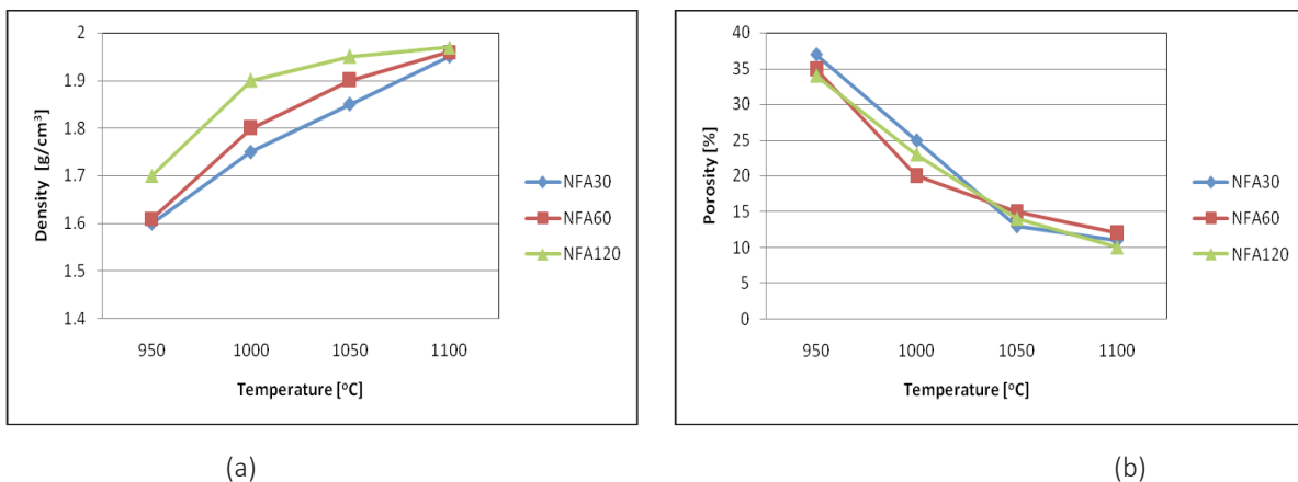
Figure 4. Physical properties of glass-ceramics sintered at different temperatures, (a) Density [g/cm 3 ]; (b) Porosity [%]
