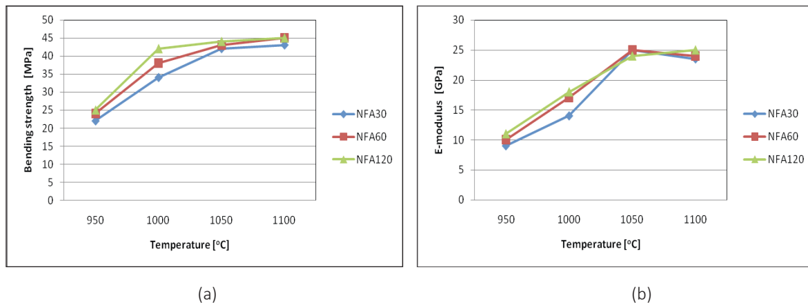
Figure 6. Mechanical properties of glass-ceramics after exposure on defined thermal treatments, a) bending strength (MPa); b) E-modulus (GPa)
