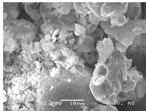
Figure 1. Morphology of raw fly ash, bar 10μm;
