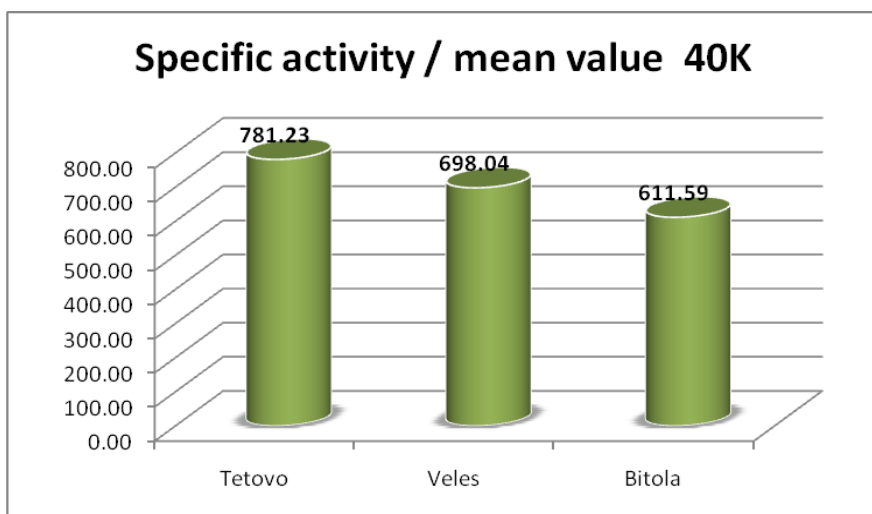
Figure 1. Mean values of the specific activities of ^{40}\text{K} in the surrounding of Skopje and three cities in Macedonia
