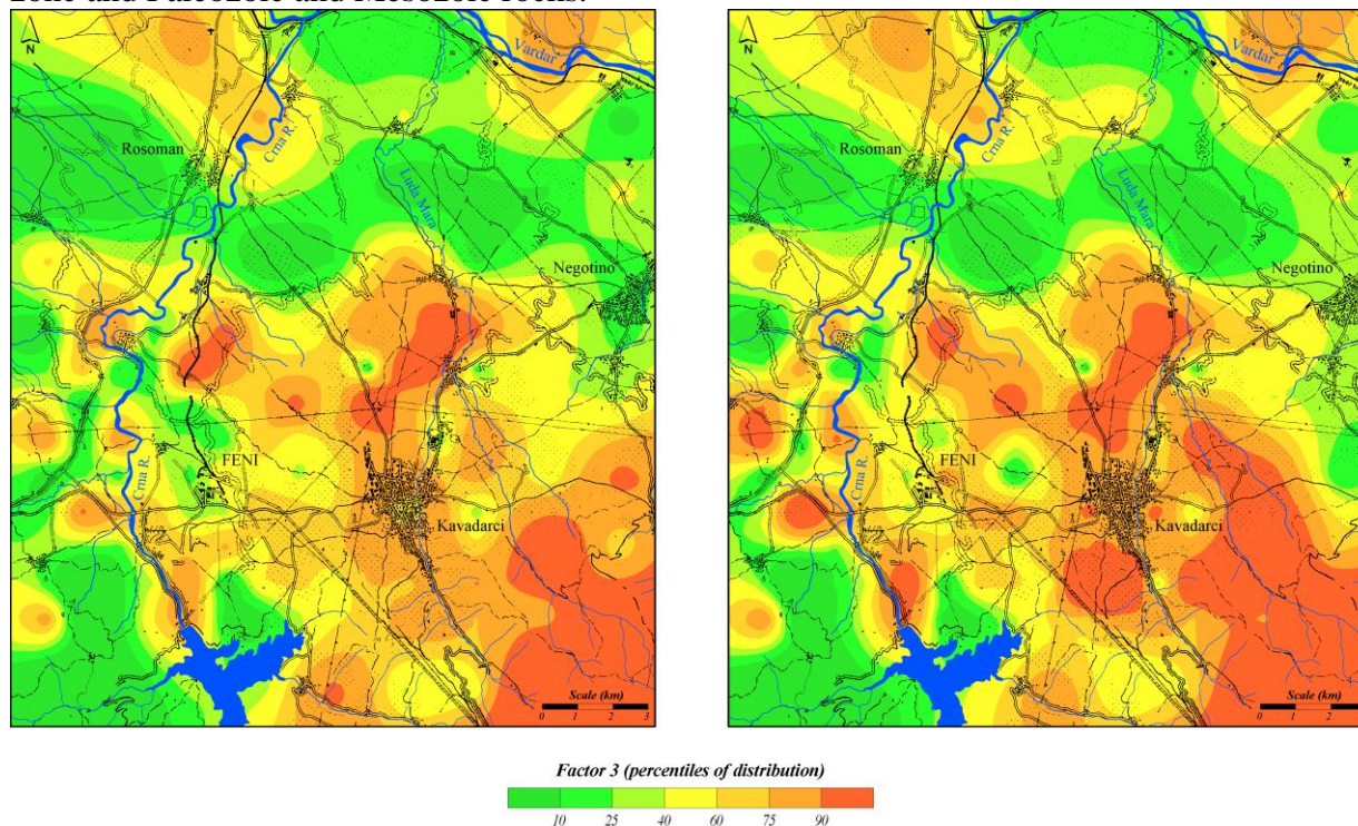
Fig. 6. Distribution of Factor 3 scores (Ba, La, Th and U) in topsoil (left) and subsoil (right)
