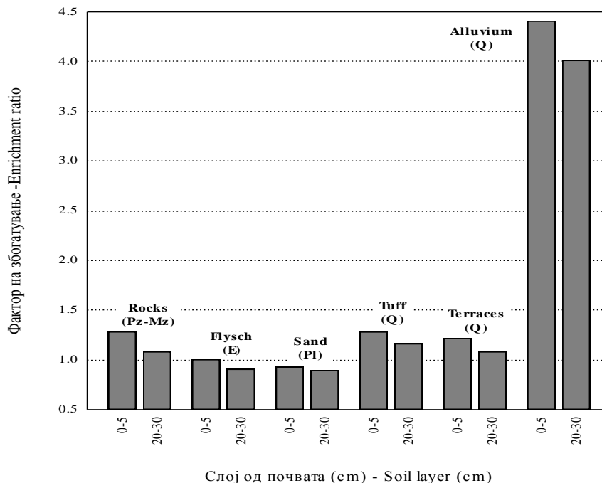
Fig. 10. Average enrichment ratios of As, Sb and Tl in topsoil (depth 0–5 cm) and subsoil (20–30 cm) versus soil average of Kavadarci regarding to basic lithological units
