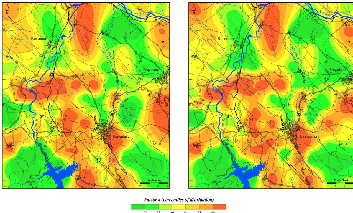
Fig. 7. Distribution of Factor 4 scores (Ca and Sr) in topsoil (left) and subsoil (right)
