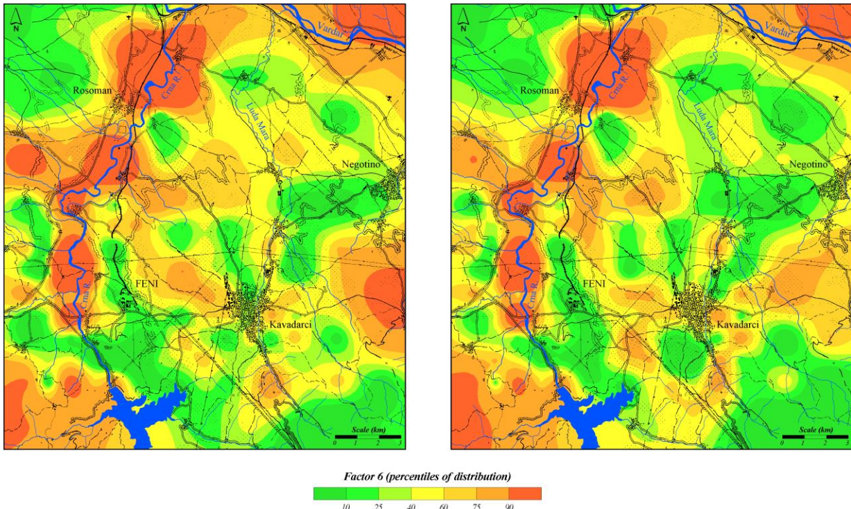
Fig. 9. Distribution of Factor 6 scores (As, Sb and Tl) in topsoil (left) and subsoil (right)
