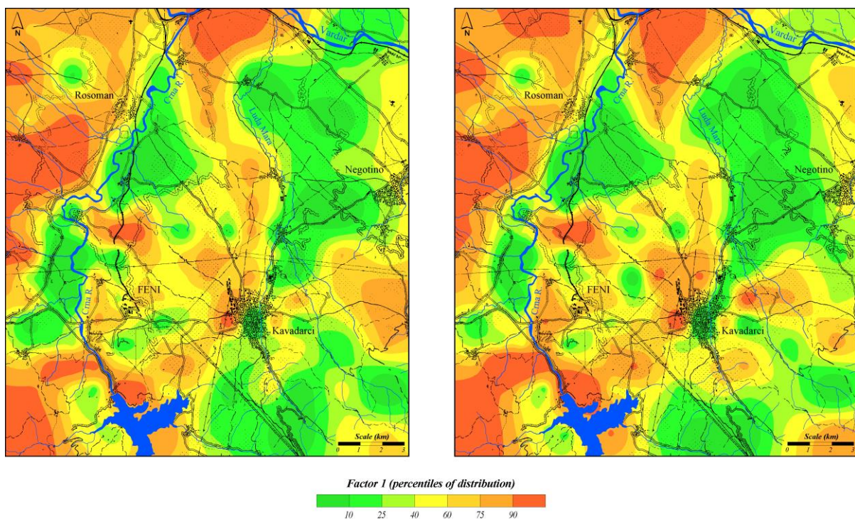
Fig. 3. Distribution of Factor 1 scores (Al, Fe, Ga, Sc and V) in topsoil (left) and subsoil (right)
