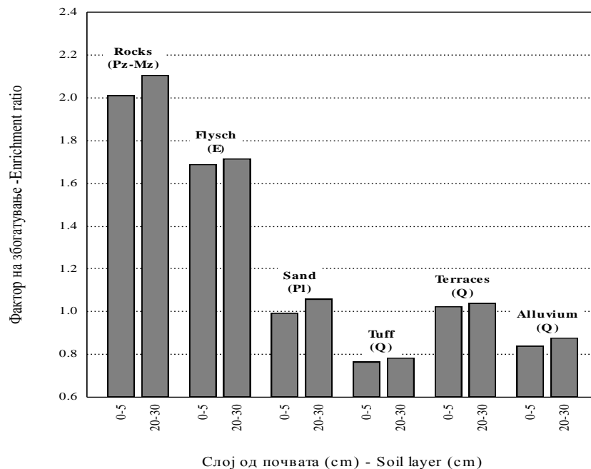
Fig. 5. Average enrichment ratios of Co, Cr, Mg and Ni in topsoil (depth 0–5 cm) and subsoil (20–30 cm) versus soil average of Kavadarci regarding to basic lithological units
