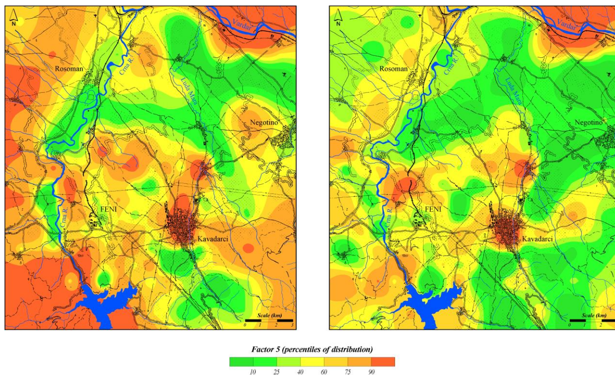
Fig. 8. Distribution of Factor 5 scores (Cd, Hg, Pb and Zn) in topsoil (left) and subsoil (right)
