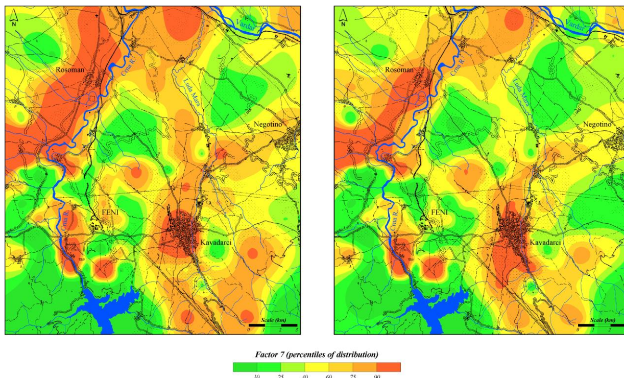
Fig. 11. Distribution of Factor 7 scores (K and P) in topsoil (left) and subsoil (right)
