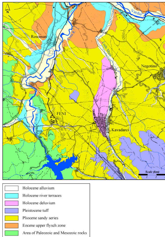
Fig. 1. Lithological map of the Kavadarci area
