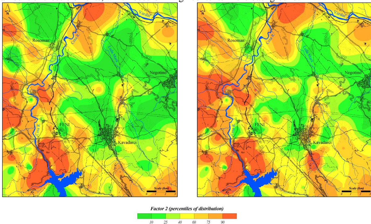
Fig. 4. Distribution of Factor 2 scores (Co, Cr, Mg and Ni) in topsoil (left) and subsoil (right)
