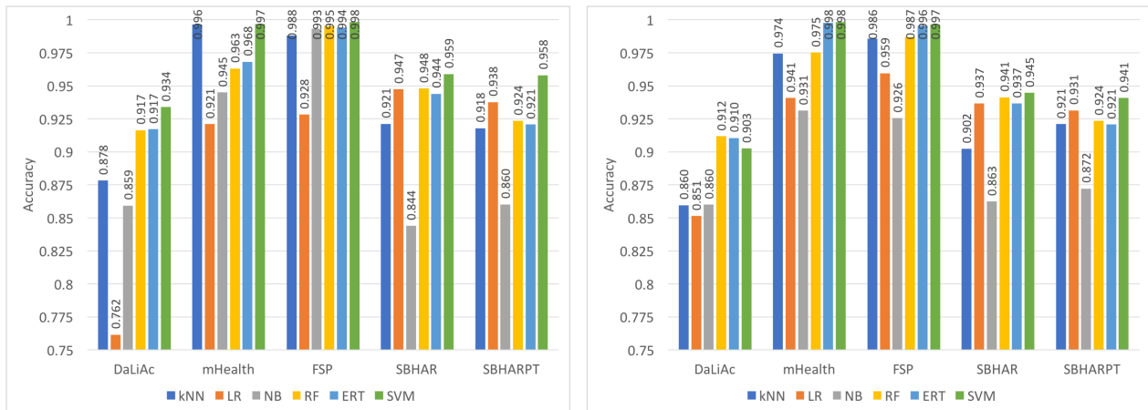
FIGURE 8. Accuracy per classification algorithm and dataset on the two final feature sets. (a) Best feature set obtained with score-drift feature screening. (b) Best feature set obtained with DFB feature selection.
