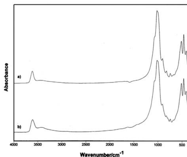
Fig. 1. FT IR spectra of muscovite from Dunje (a) and Nežilovo (b) obtained using KBr pellets.
