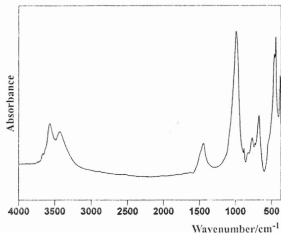
FT IR spectrum of kosmatite
