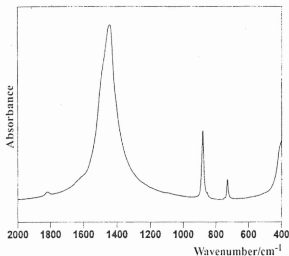
FT IR spectrum of dolomite
