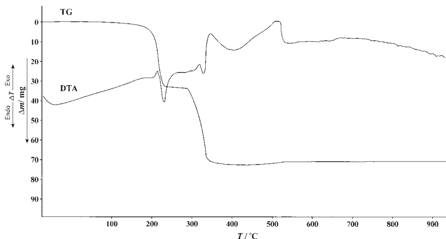
Fig. 2 TG and DTA curves of hydroxylammonium uranyl acetate ( m=171.00 mg)
