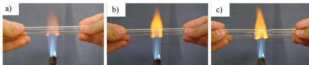
Figure 1. Demonstration of ampoule preparation: a) the test tube of standard dimensions (16 × 160 mm) is heated while rotated; b) when the glass softens the test tube is pulled by both ends; c) once the required neck length is achieved, the test tube (now ampoule) is pulled out of the flame.
