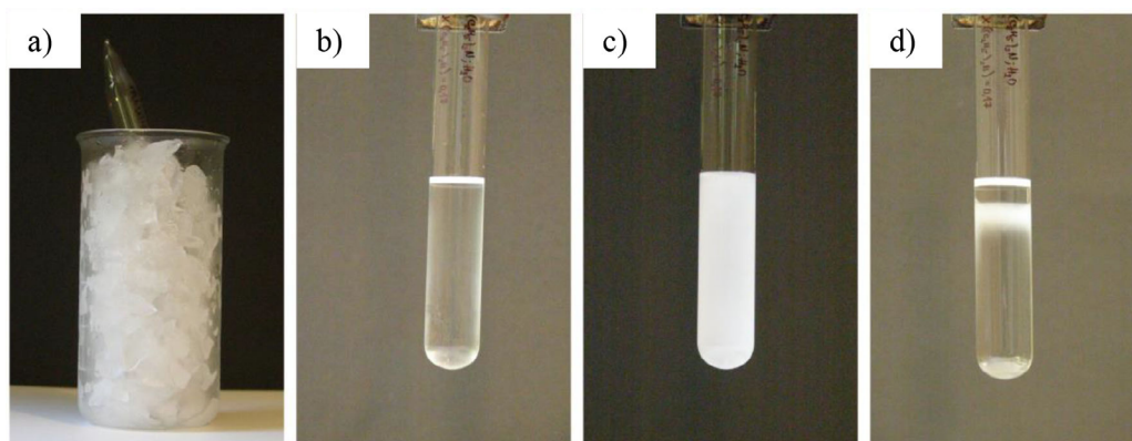
Figure 3. System with LCST, binary mixture of: (\text{C}_2\text{H}_5)_3\text{N-H}_2\text{O} . After being cooled, (a) the system becomes homogeneous (b) and when it reaches the critical temperature, it becomes opalescent (c). After few minutes, the system separates in two phases (d).
