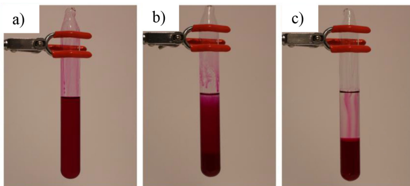
Figure 5. It was determined that phenolphthalein is an excellent colorant for the system (\text{C}_2\text{H}_5)_3\text{N-H}_2\text{O} since it colors only the water layer while the organic layer stays colorless after the system reaches the critical temperature: a) after the system is cooled at 4.3 °C it becomes homogeneous; b) when left at room temperature two layers start to form; c) after few minutes the separation is (more or less) complete.
