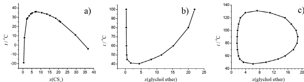
Figure 4. Diagrams representing systems with a) UCST, \text{CS}_2\text{-CH}_3\text{OH} (McKelvy and Simpson, 1922), b) LCST, diethylene glycol n -pentyl ether–water, c) both upper and lower critical solution temperature, ethylene glycole n -butyl ether–water (Christensen et al., 2005).
