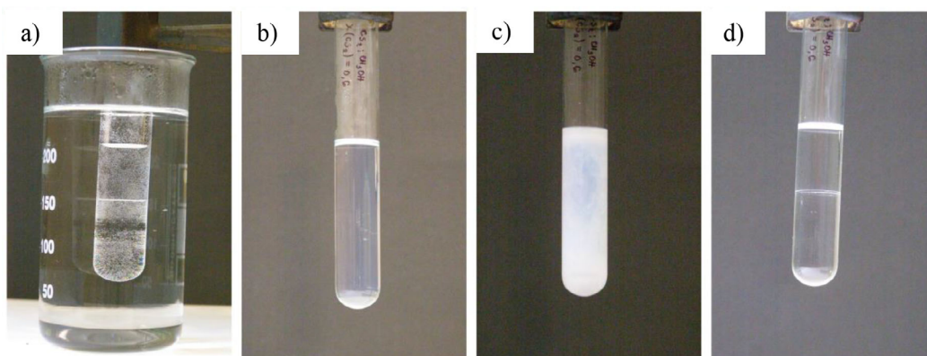
Figure 2. System with UCST, binary mixture of: \text{CS}_2\text{-CH}_3\text{OH} . After being heated, (a) the system becomes homogeneous (b) and when it reaches the critical temperature, it becomes opalescent (c). After few minutes, the system separates in two layers (d).
