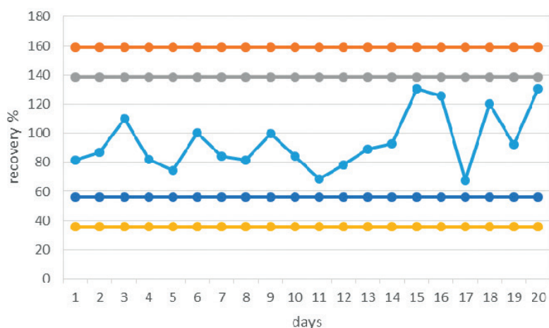
Figure 3. Shewhart control chart for AFB_1 (spiking level 0.50 \mu\text{g}/\text{kg} )
