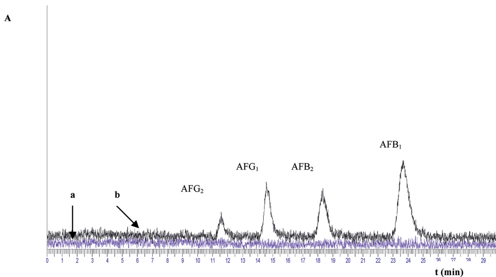
Figure 1. Chromatograms of (a) blank liver sample and (b) fortified liver sample with concentration of AFB 1 0.50 \mu\text{g}/\text{kg} ; AFB 2 0.142 \mu\text{g}/\text{kg} ; AFG 1 0.517 \mu\text{g}/\text{kg} and AFG 2 0.166 \mu\text{g}/\text{kg}
