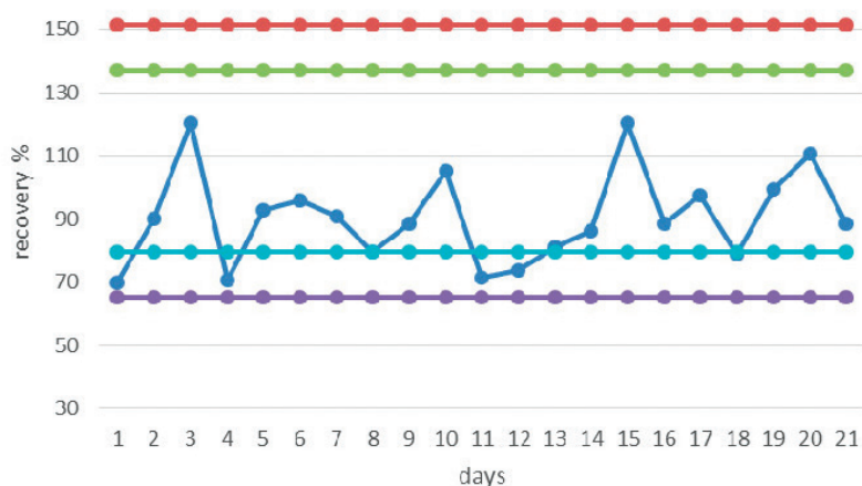
Figure 4. Shewhart control chart for OTA (spiking level 5 \mu\text{g}/\text{kg} )
