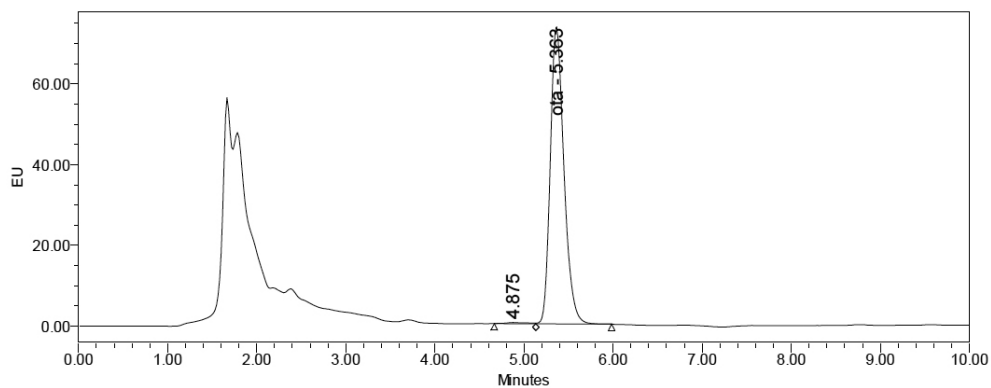
Figure 2. Chromatogram of fortified liver sample with concentration of OTA 5.0 \mu\text{g}/\text{kg}
