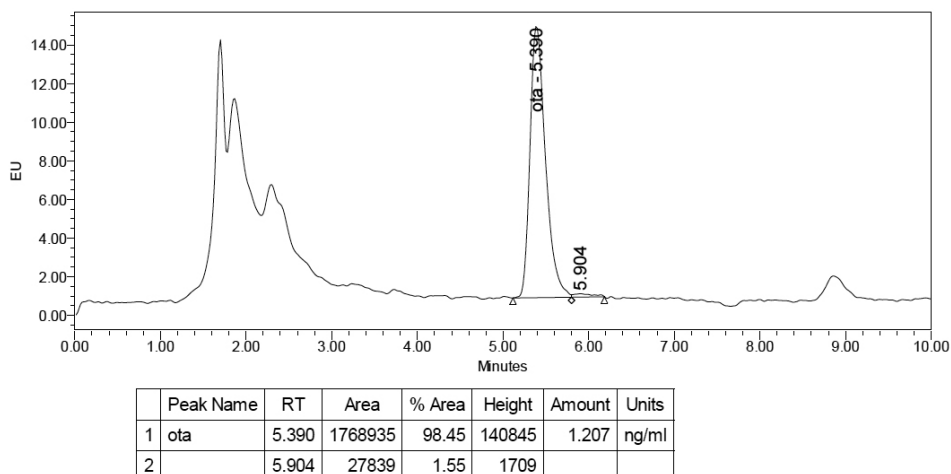
Figure 5. Chromatogram of liver sample with concentration of OTA 0.86 \mu\text{g}/\text{kg} (dilution factor is 1.4)
