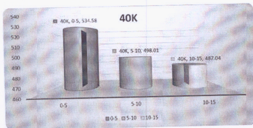
Fig. 3. Mean values of specific activities of 40 K at different depths
