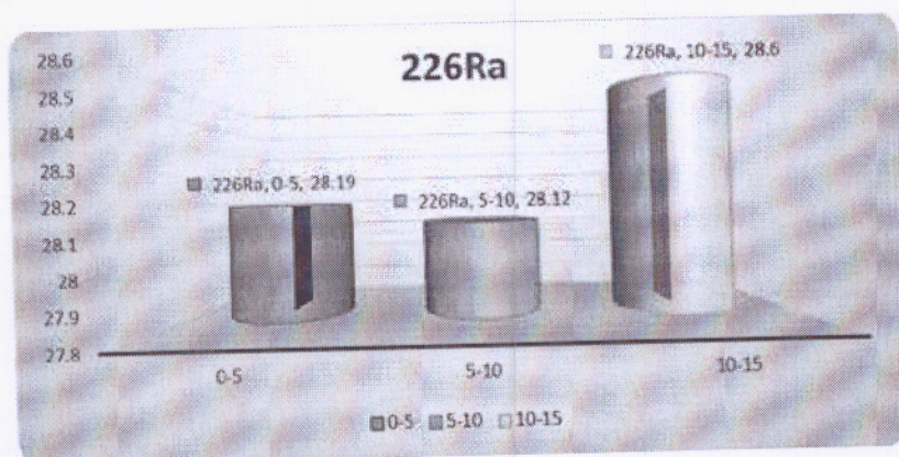
Fig. 1. Mean values of specific activities of ^{226}\text{Ra} at different depths
