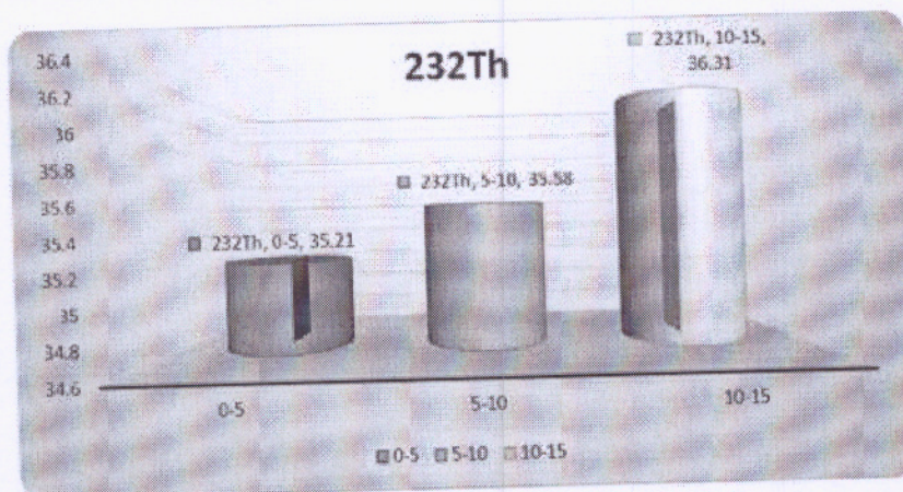
Fig. 2. Mean values of specific activities of ^{232}\text{Th} at different depths
